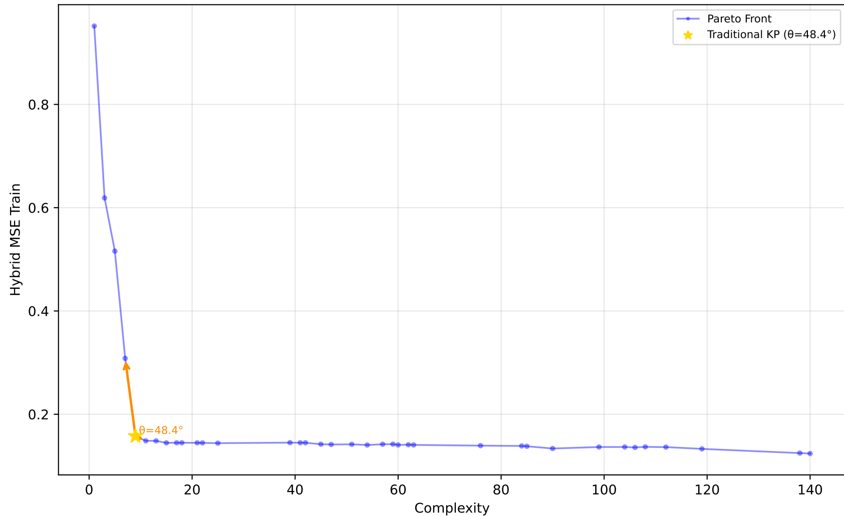
529_pollen - Run 3 - MVP - Hybrid MSE Train \lambda_1=0.90, \lambda_2=0.00, \lambda_3=0.00 | Difficulty: 1.00 | Method: hmr
