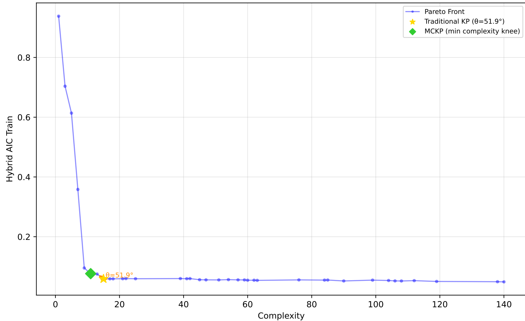
529_pollen - Run 3 - SVP - Hybrid AIC Train \lambda_1=0.10 , \lambda_2=0.80 , \lambda_3=0.30 | Difficulty: 1.00 | Method: hmr
