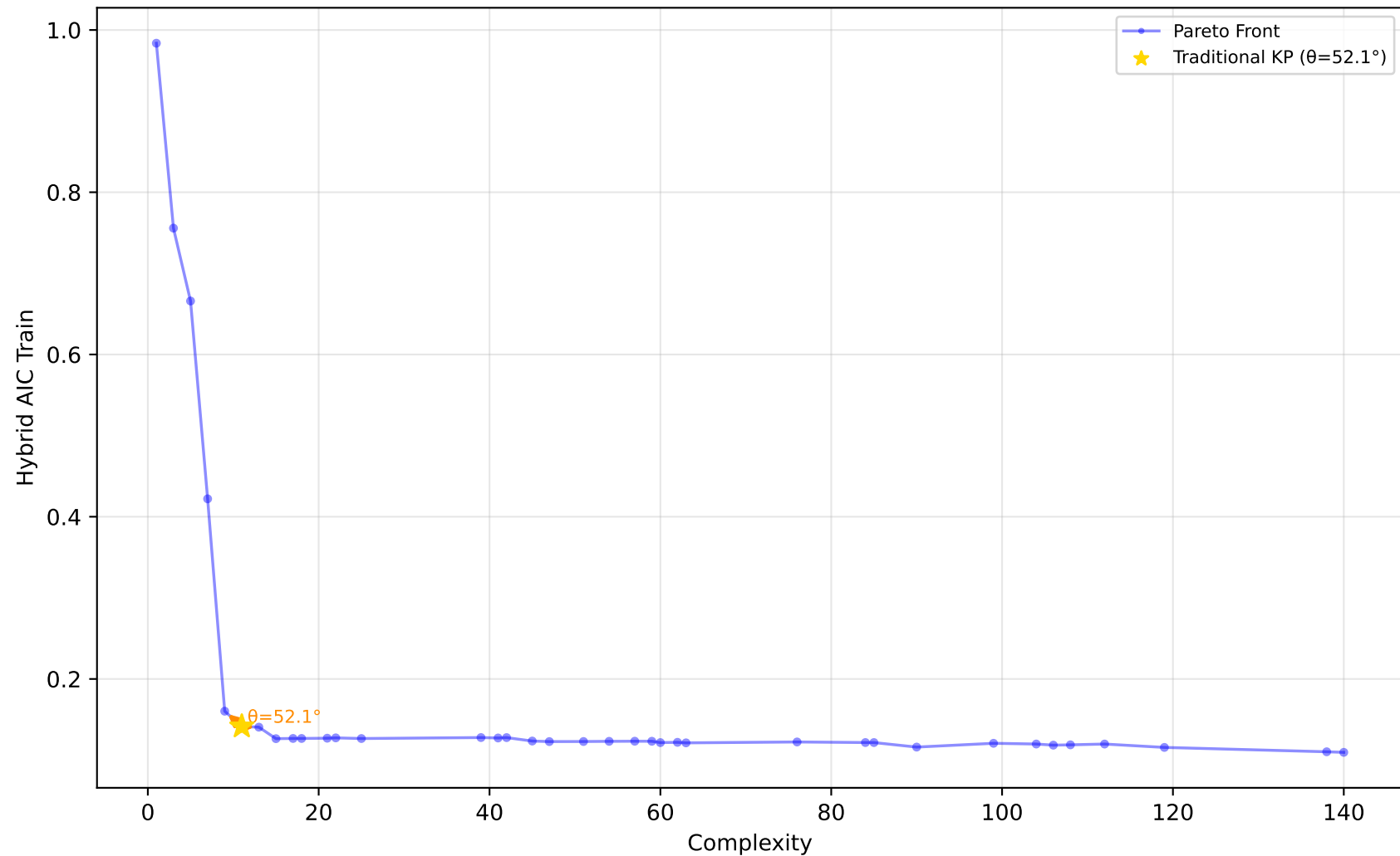
529_pollen - Run 3 - SVP - Hybrid AIC Train \lambda_1=0.60, \lambda_2=0.40, \lambda_3=1.00 | Difficulty: 1.00 | Method: hmr
