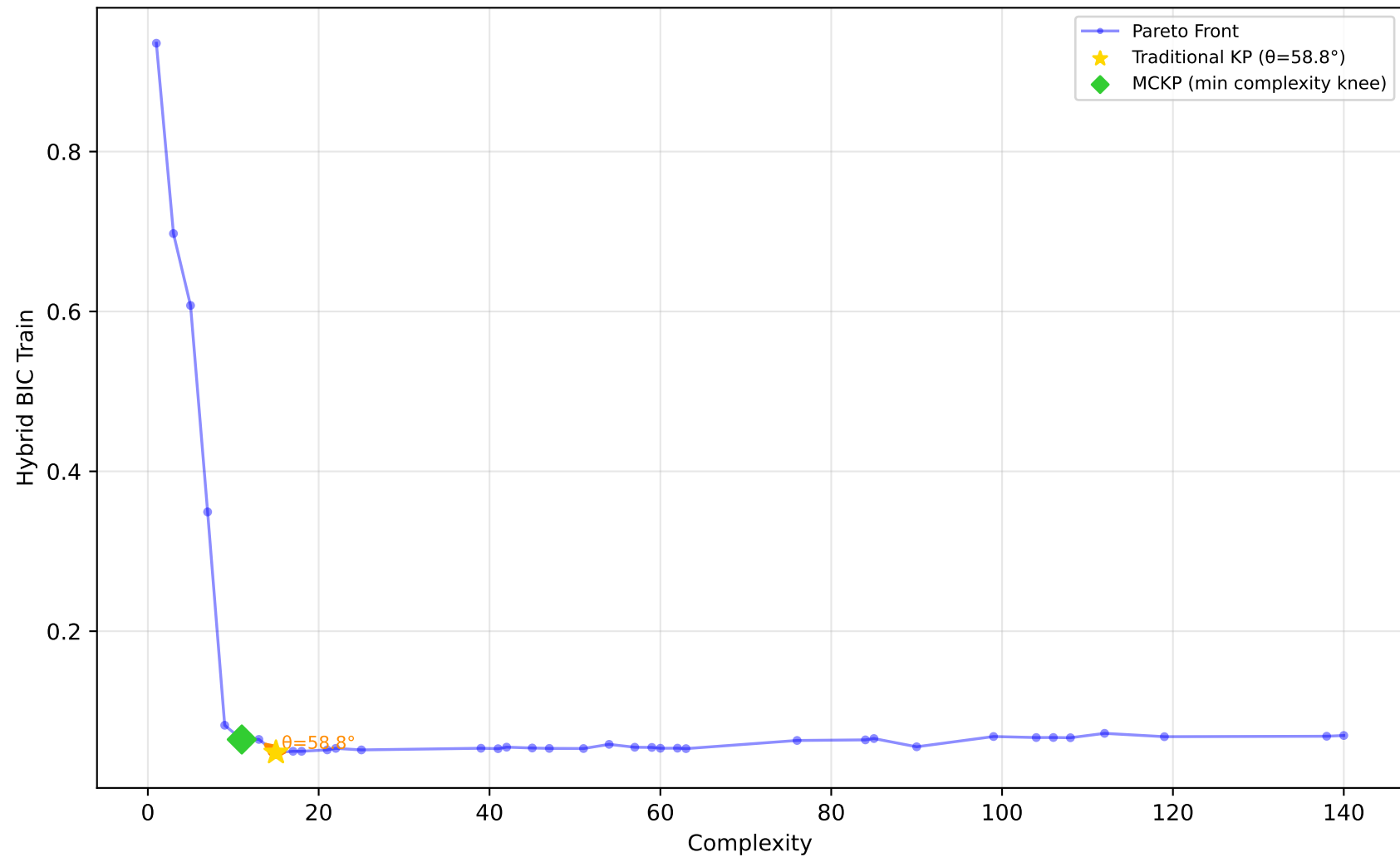
529_pollen - Run 3 - SVP - Hybrid BIC Train \lambda_1=0.10, \lambda_2=0.80, \lambda_3=0.30 | Difficulty: 1.00 | Method: hmr
