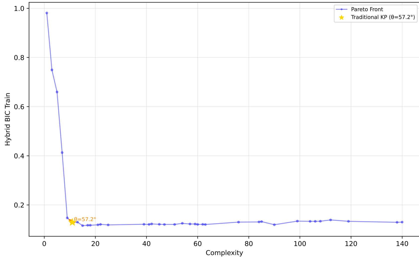
529_pollen - Run 3 - SVP - Hybrid BIC Train \lambda_1=0.60, \lambda_2=0.40, \lambda_3=1.00 | Difficulty: 1.00 | Method: hmr
