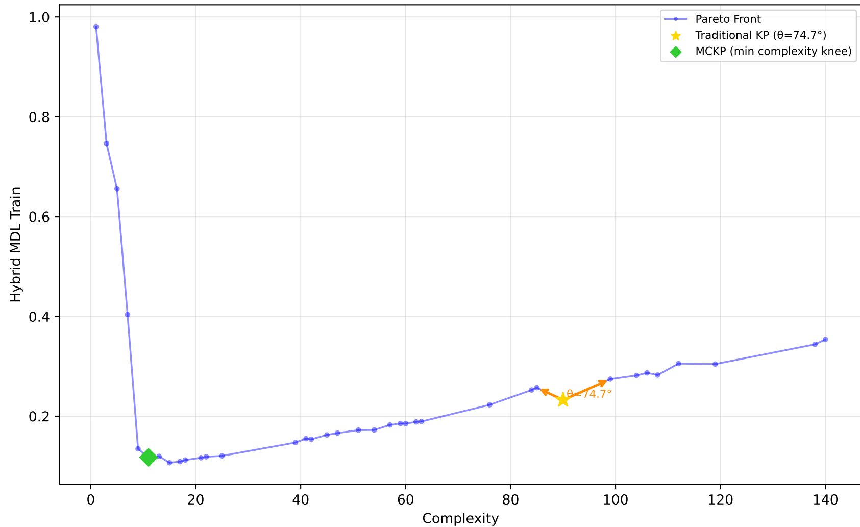
529_pollen - Run 3 - SVP - Hybrid MDL Train \lambda_1=0.60, \lambda_2=0.40, \lambda_3=1.00 | Difficulty: 1.00 | Method: hmr
