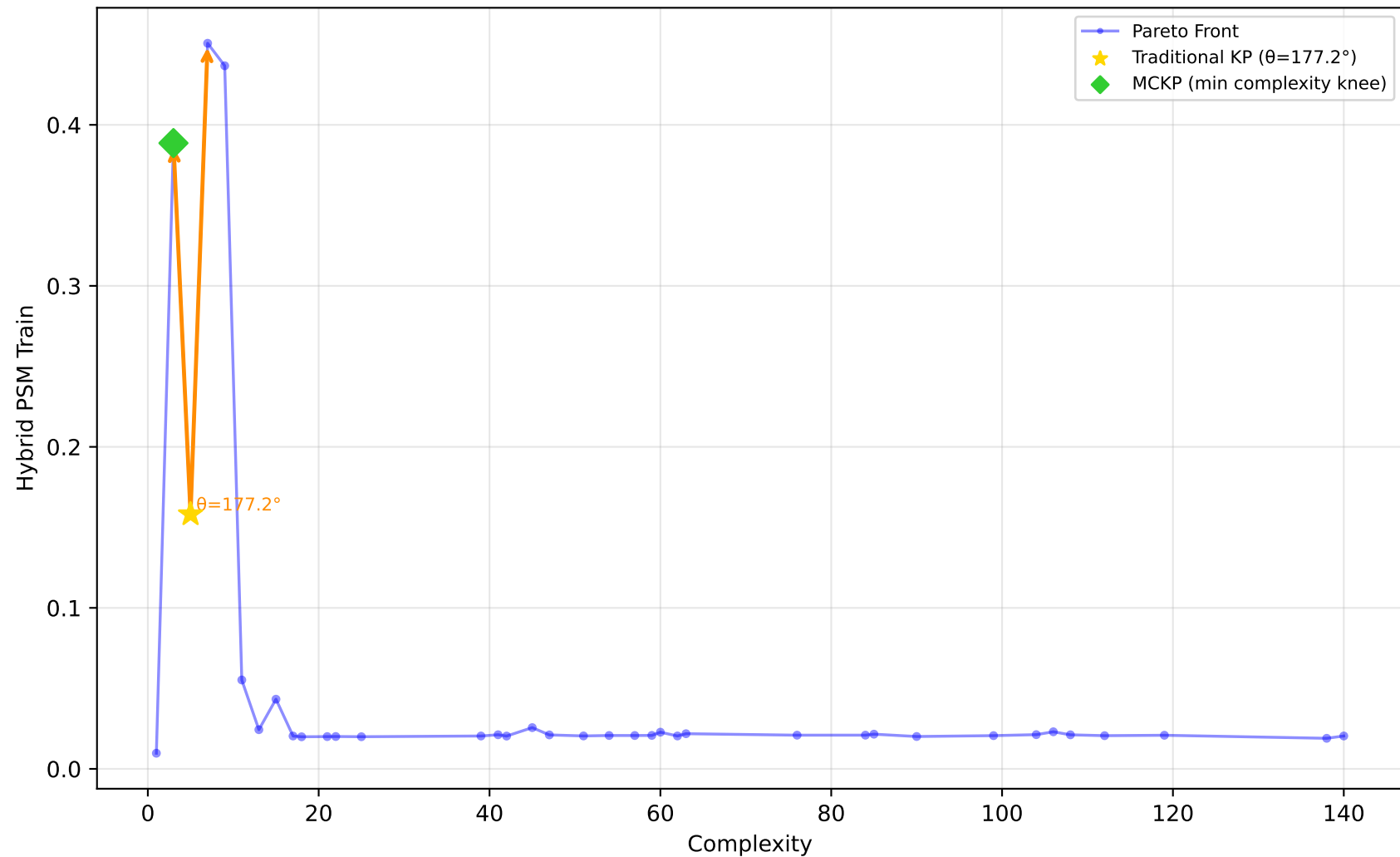
529_pollen - Run 3 - SVP - Hybrid PSM Train \lambda_1=0.10, \lambda_2=0.80, \lambda_3=0.30 | Difficulty: 1.00 | Method: hmr
