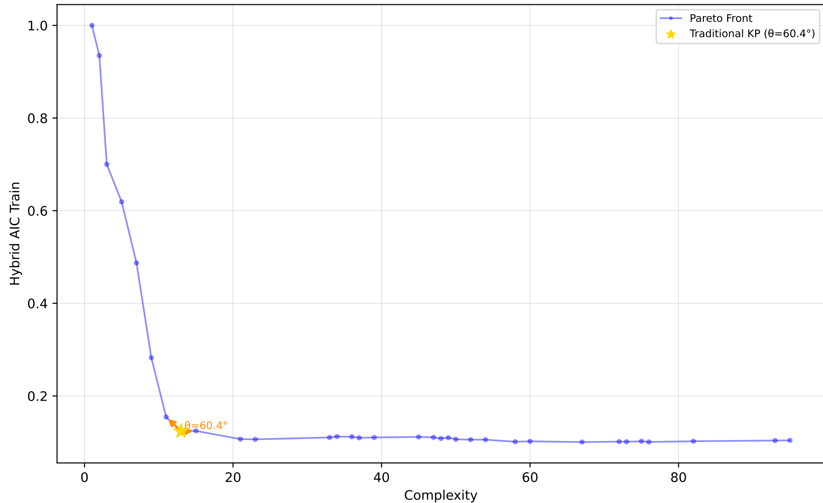
529_pollen - Run 4 - MVP - Hybrid AIC Train \lambda_1=0.00, \lambda_2=1.00, \lambda_3=0.80 | Difficulty: 1.00 | Method: hmr
