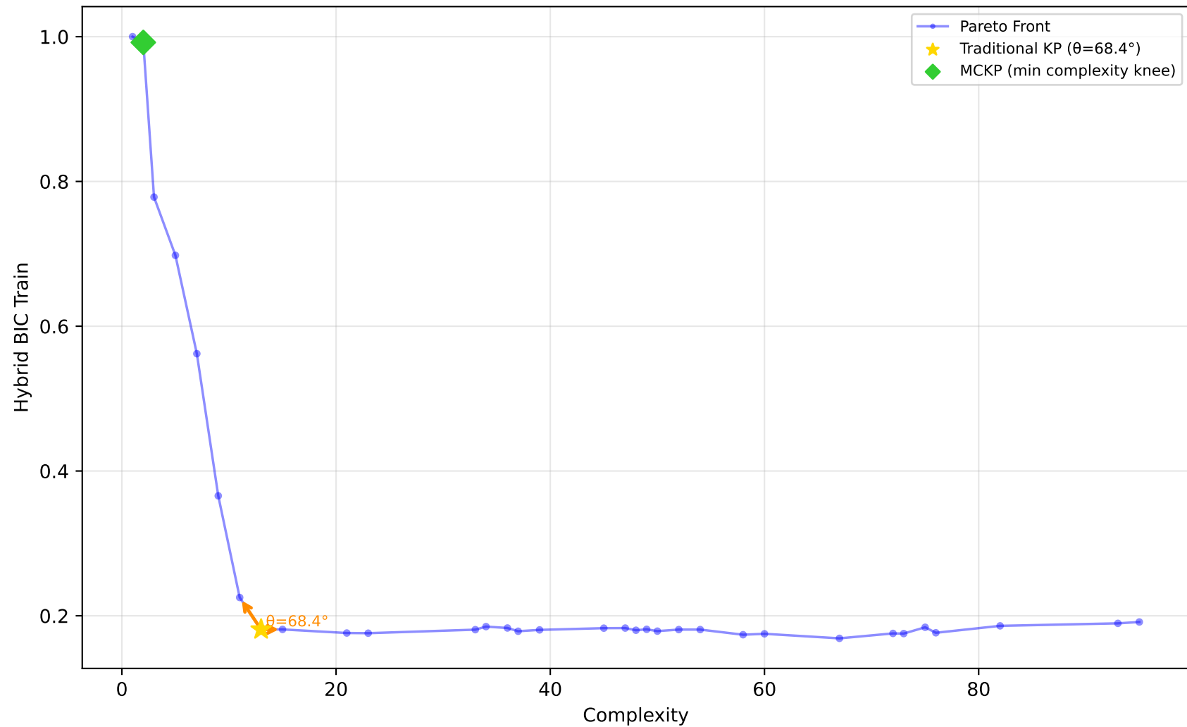
529_pollen - Run 4 - MVP - Hybrid BIC Train \lambda_1=0.90, \lambda_2=0.00, \lambda_3=0.00 | Difficulty: 1.00 | Method: hmr
