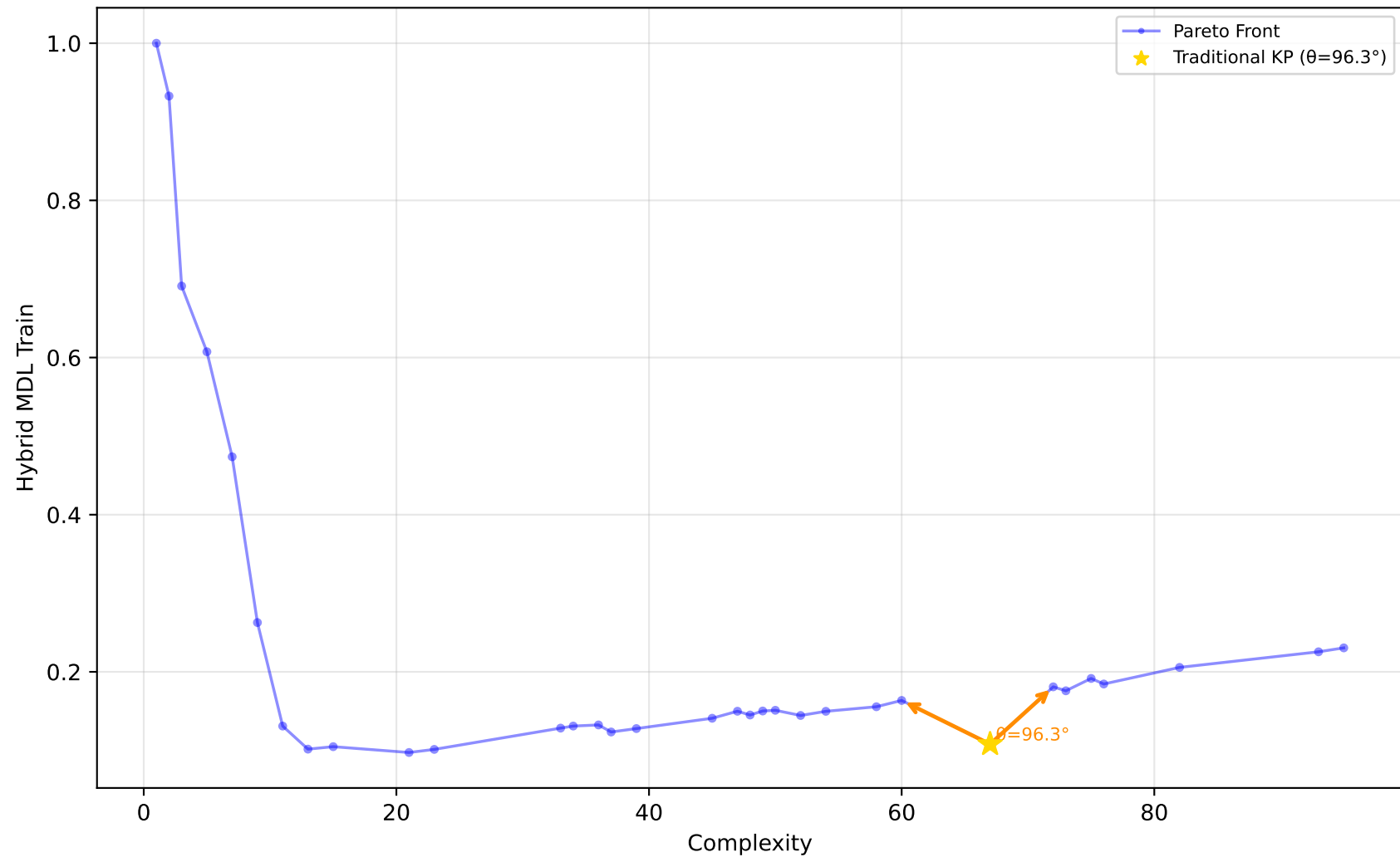
529_pollen - Run 4 - MVP - Hybrid MDL Train \lambda_1=0.00, \lambda_2=1.00, \lambda_3=0.80 | Difficulty: 1.00 | Method: hmr
