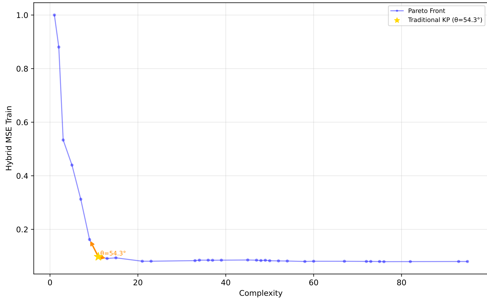
529_pollen - Run 4 - MVP - Hybrid MSE Train \lambda_1=0.00, \lambda_2=1.00, \lambda_3=0.80 | Difficulty: 1.00 | Method: hmr
