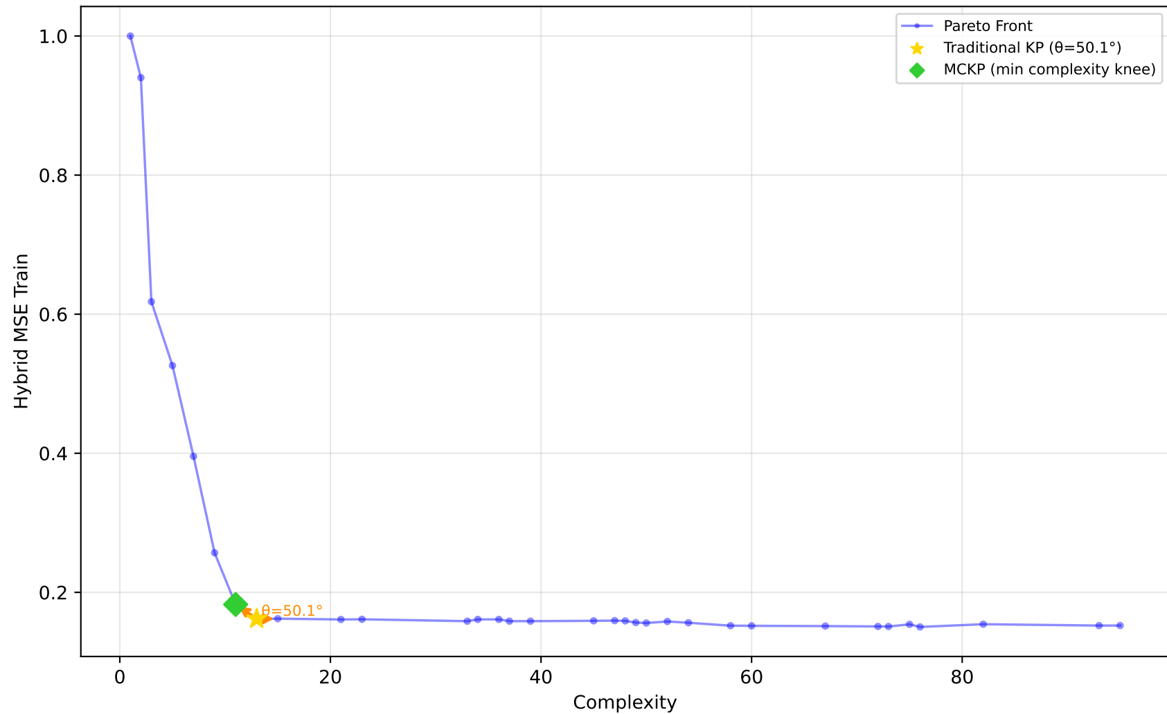
529_pollen - Run 4 - MVP - Hybrid MSE Train \lambda_1=0.90, \lambda_2=0.00, \lambda_3=0.00 | Difficulty: 1.00 | Method: hmr
