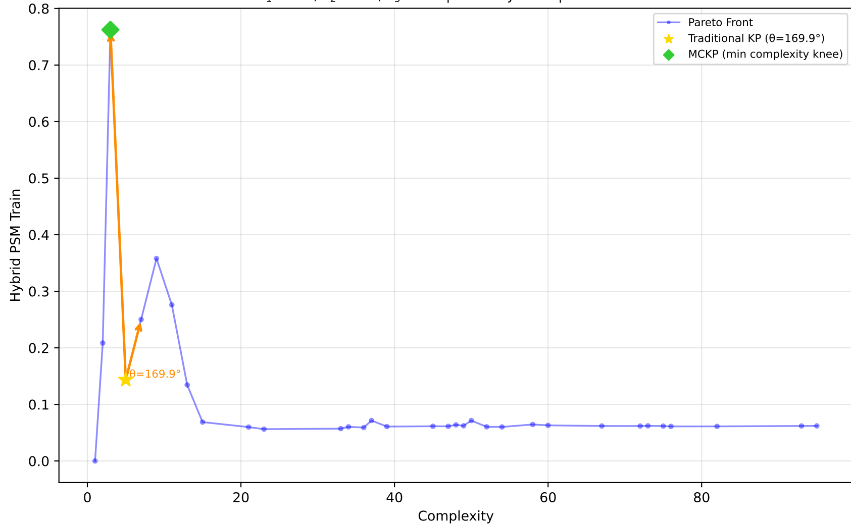
529_pollen - Run 4 - MVP - Hybrid PSM Train \lambda_1=0.00, \lambda_2=1.00, \lambda_3=0.80 | Difficulty: 1.00 | Method: hmr
