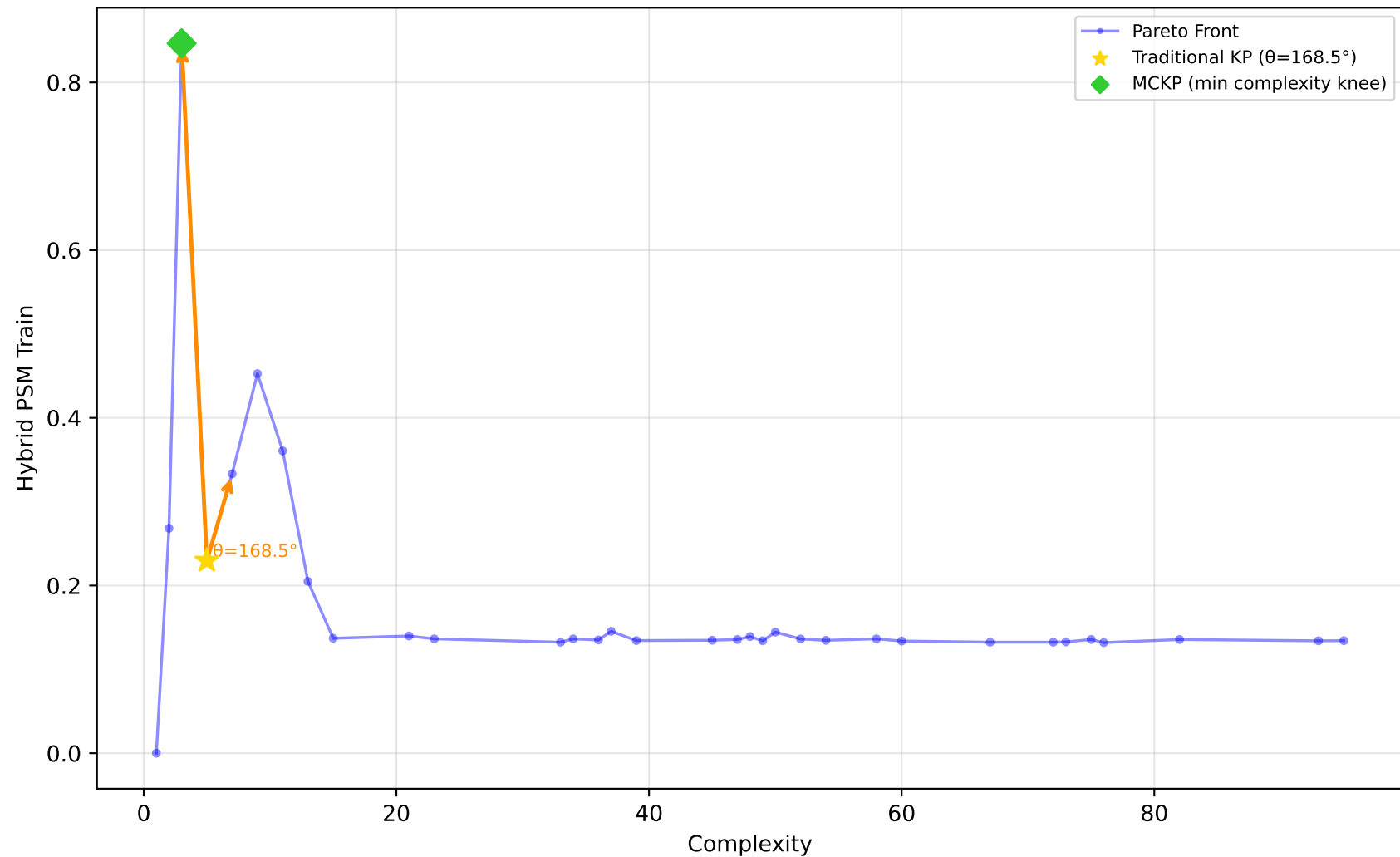
529_pollen - Run 4 - MVP - Hybrid PSM Train \lambda_1=0.90, \lambda_2=0.00, \lambda_3=0.00 | Difficulty: 1.00 | Method: hmr
