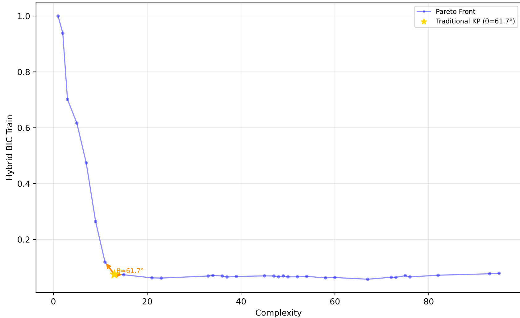
529_pollen - Run 4 - SVP - Hybrid BIC Train \lambda_1=0.10, \lambda_2=0.80, \lambda_3=0.30 | Difficulty: 1.00 | Method: hmr
