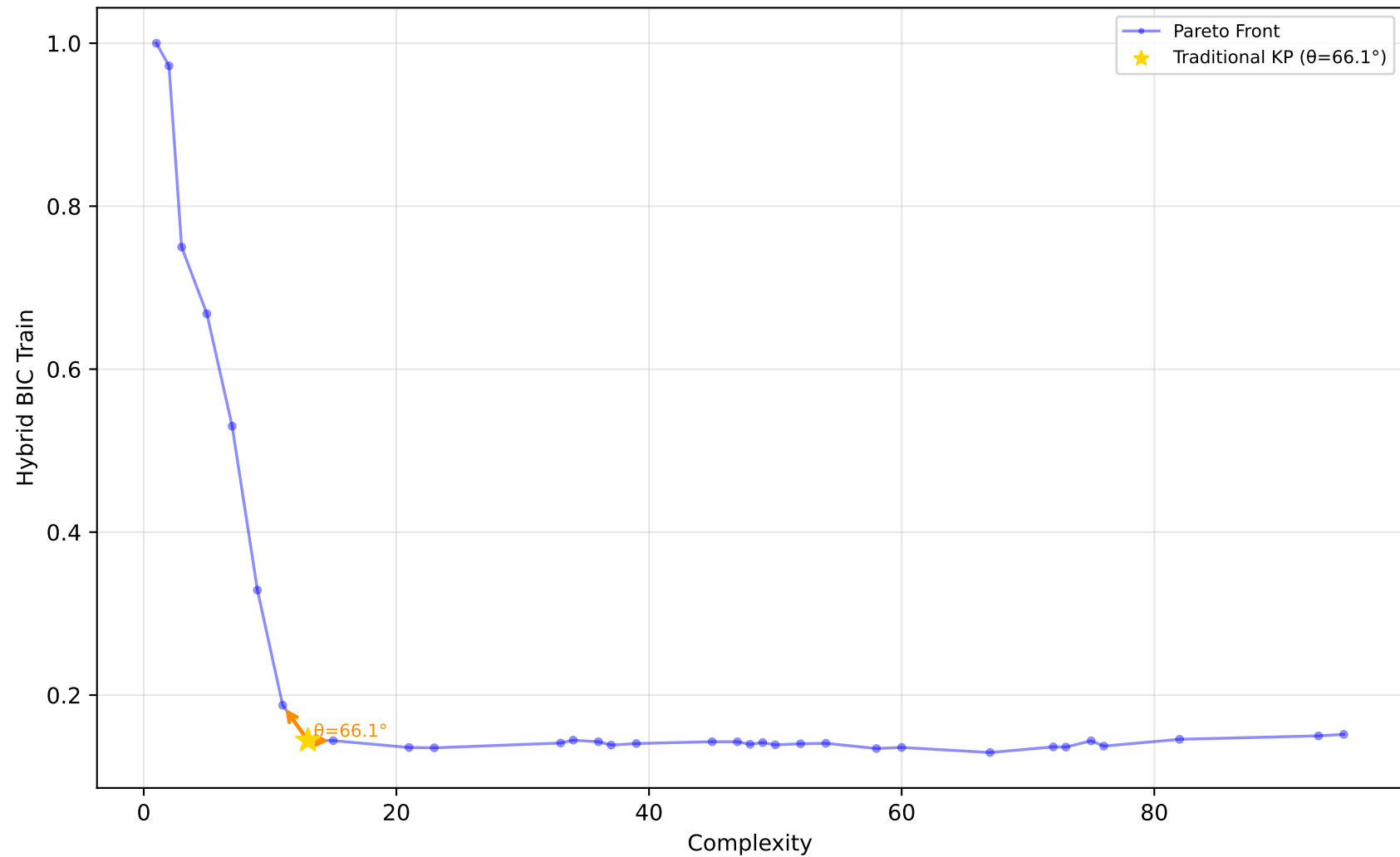
529_pollen - Run 4 - SVP - Hybrid BIC Train \lambda_1=0.60, \lambda_2=0.40, \lambda_3=1.00 | Difficulty: 1.00 | Method: hmr
