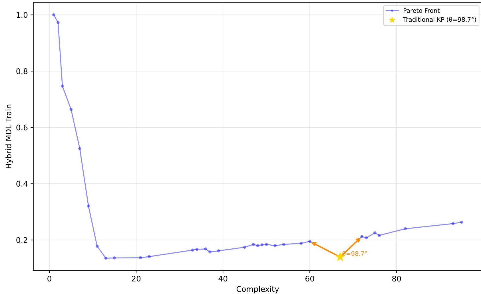
529_pollen - Run 4 - SVP - Hybrid MDL Train \lambda_1=0.60, \lambda_2=0.40, \lambda_3=1.00 | Difficulty: 1.00 | Method: hmr
