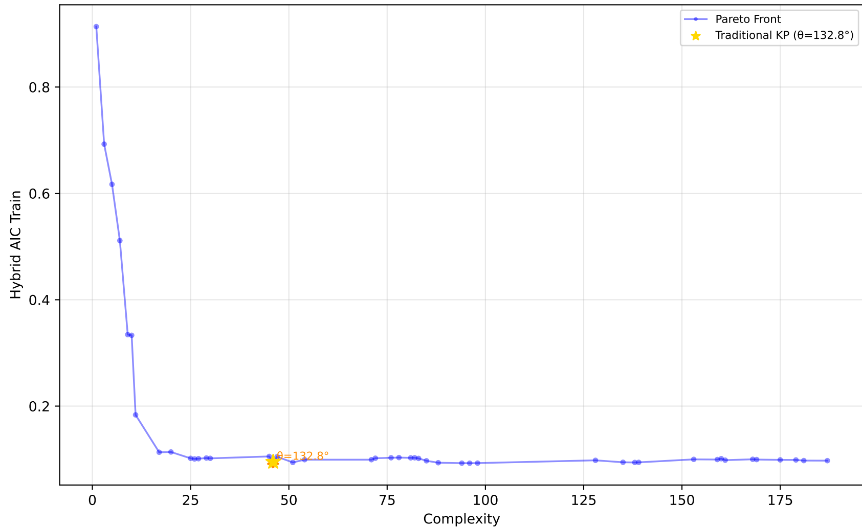
529_pollen - Run 5 - MVP - Hybrid AIC Train \lambda_1=0.00 , \lambda_2=1.00 , \lambda_3=0.80 | Difficulty: 1.00 | Method: hmr
