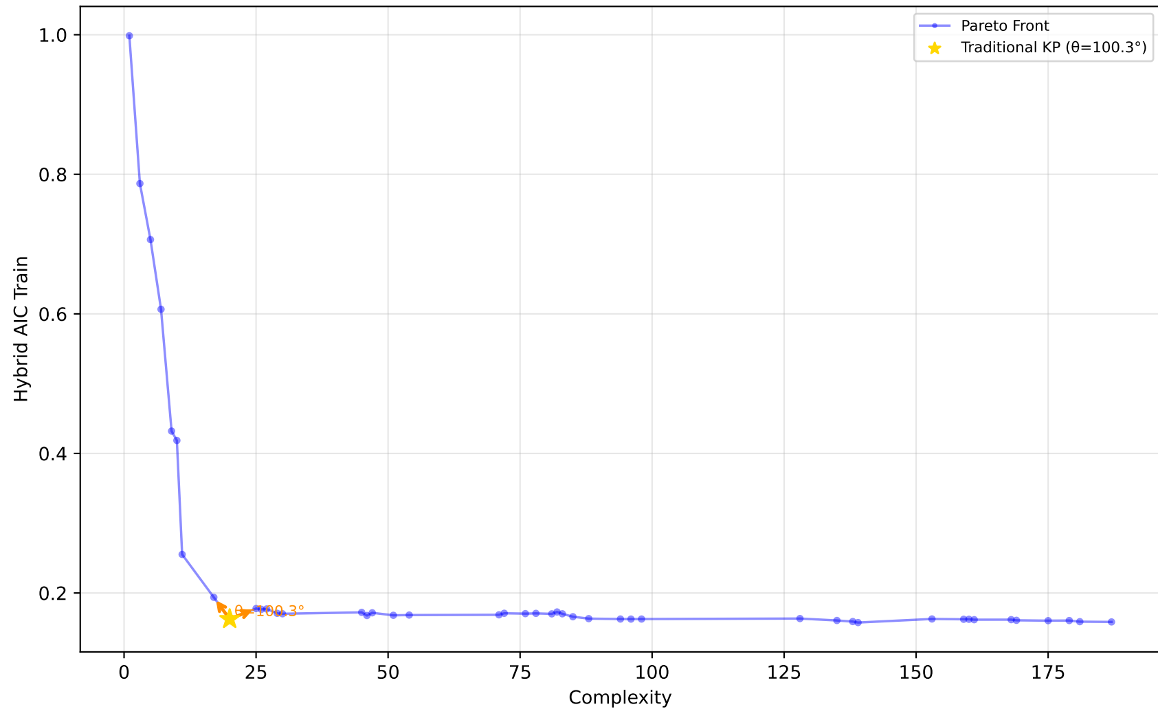
529_pollen - Run 5 - MVP - Hybrid AIC Train \lambda_1=0.90, \lambda_2=0.00, \lambda_3=0.00 | Difficulty: 1.00 | Method: hmr
