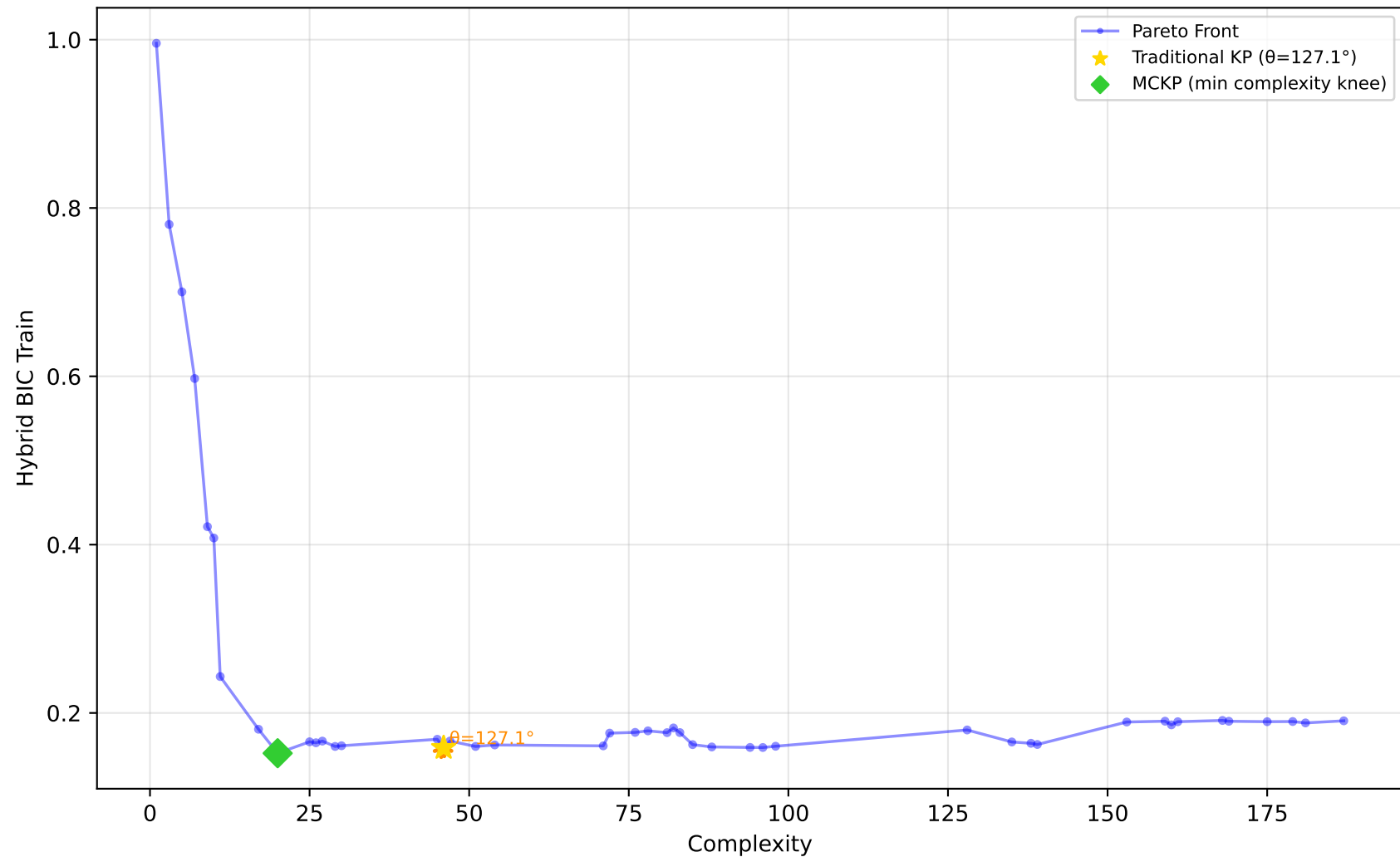
529_pollen - Run 5 - MVP - Hybrid BIC Train \lambda_1=0.90, \lambda_2=0.00, \lambda_3=0.00 | Difficulty: 1.00 | Method: hmr
