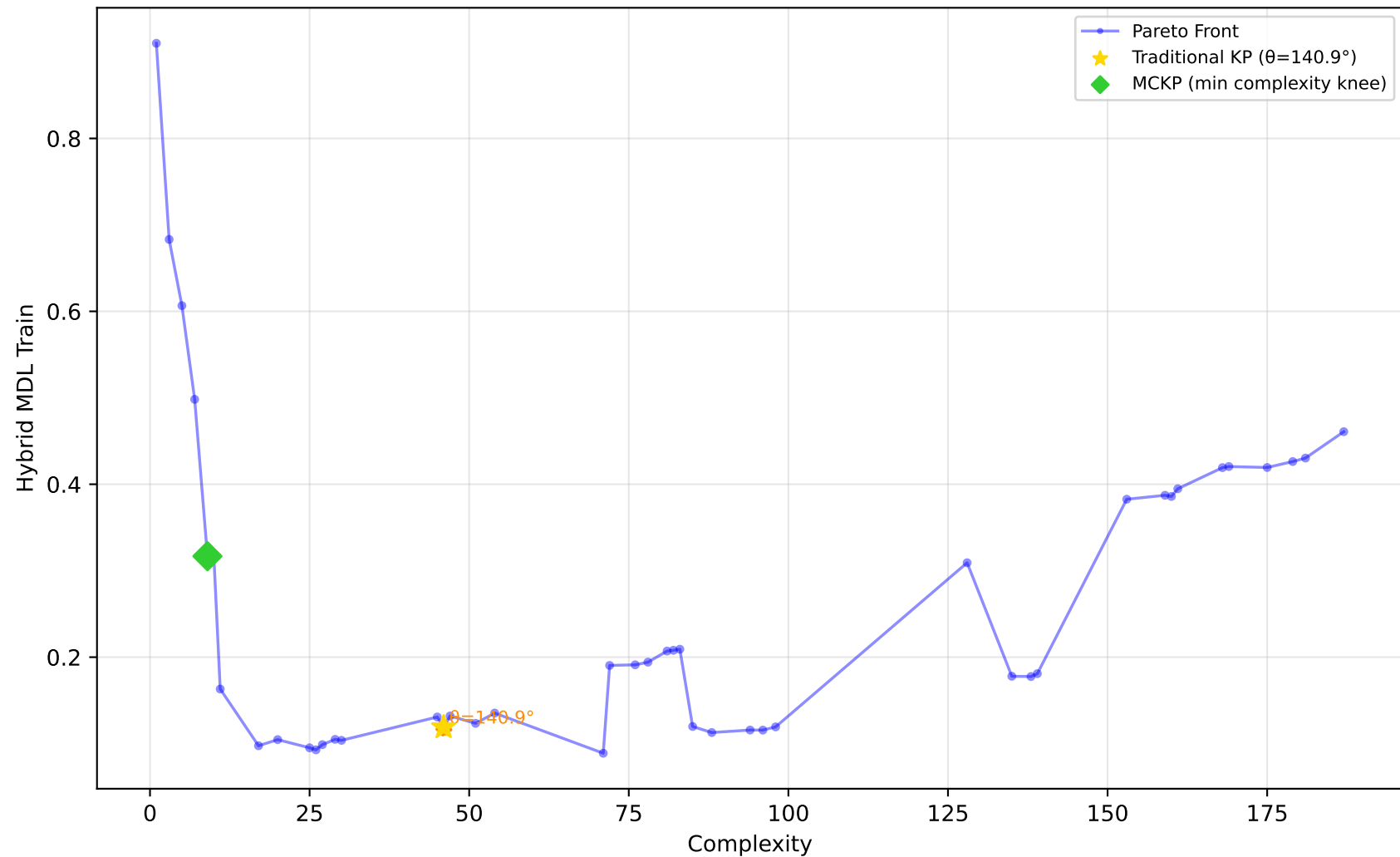
529_pollen - Run 5 - MVP - Hybrid MDL Train \lambda_1=0.00, \lambda_2=1.00, \lambda_3=0.80 | Difficulty: 1.00 | Method: hmr
