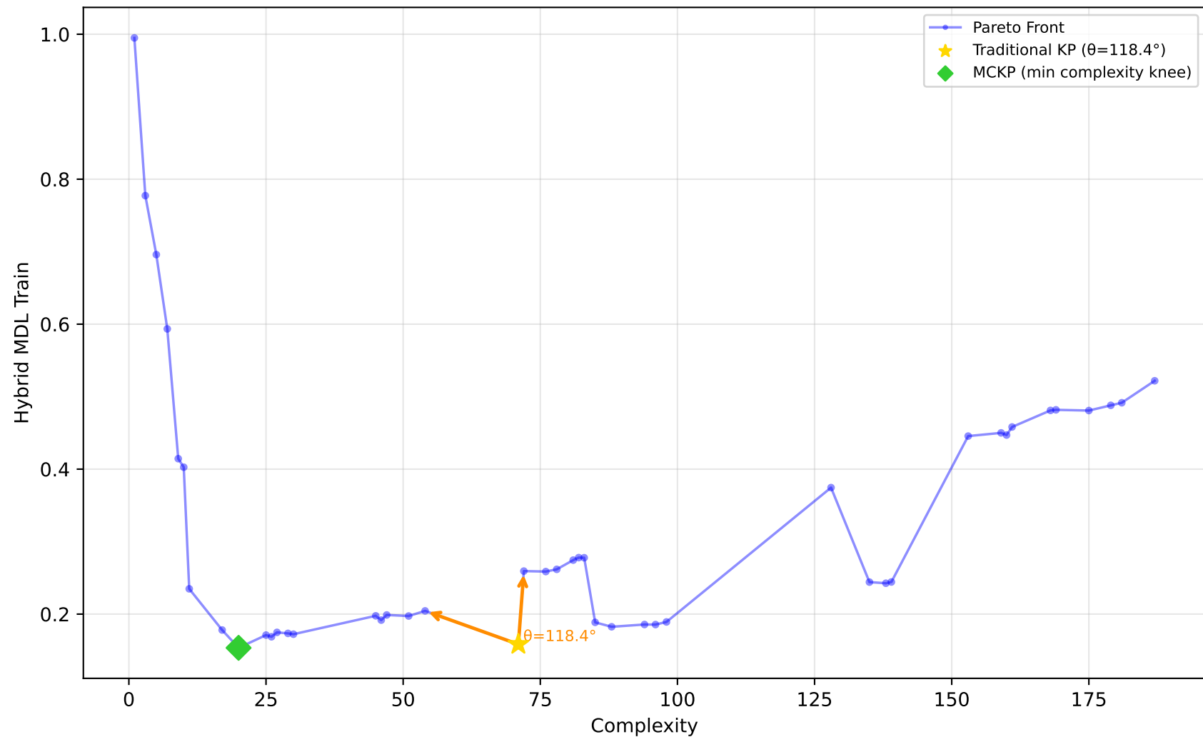
529_pollen - Run 5 - MVP - Hybrid MDL Train \lambda_1=0.90, \lambda_2=0.00, \lambda_3=0.00 | Difficulty: 1.00 | Method: hmr
