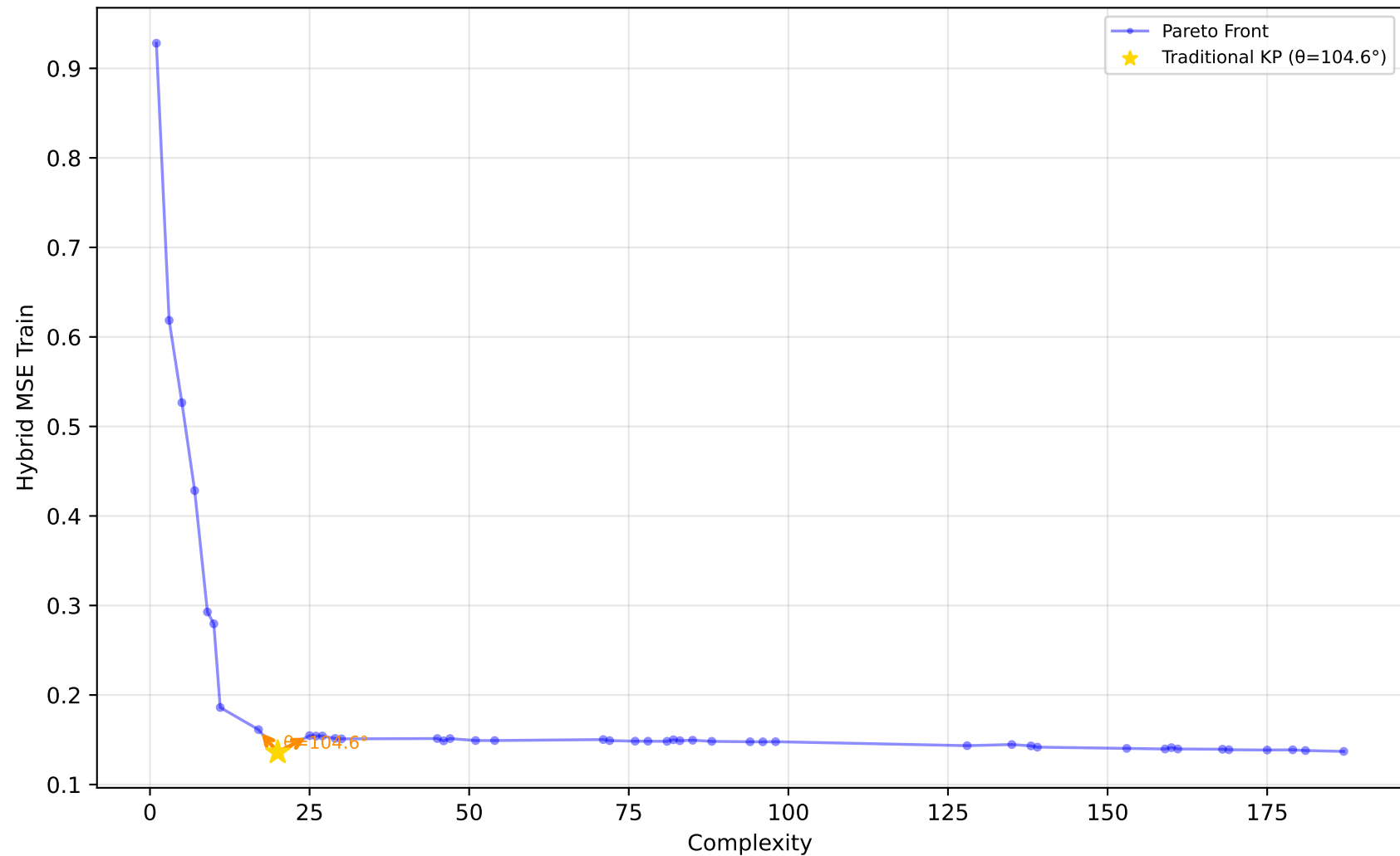
529_pollen - Run 5 - MVP - Hybrid MSE Train \lambda_1=0.90, \lambda_2=0.00, \lambda_3=0.00 | Difficulty: 1.00 | Method: hmr
