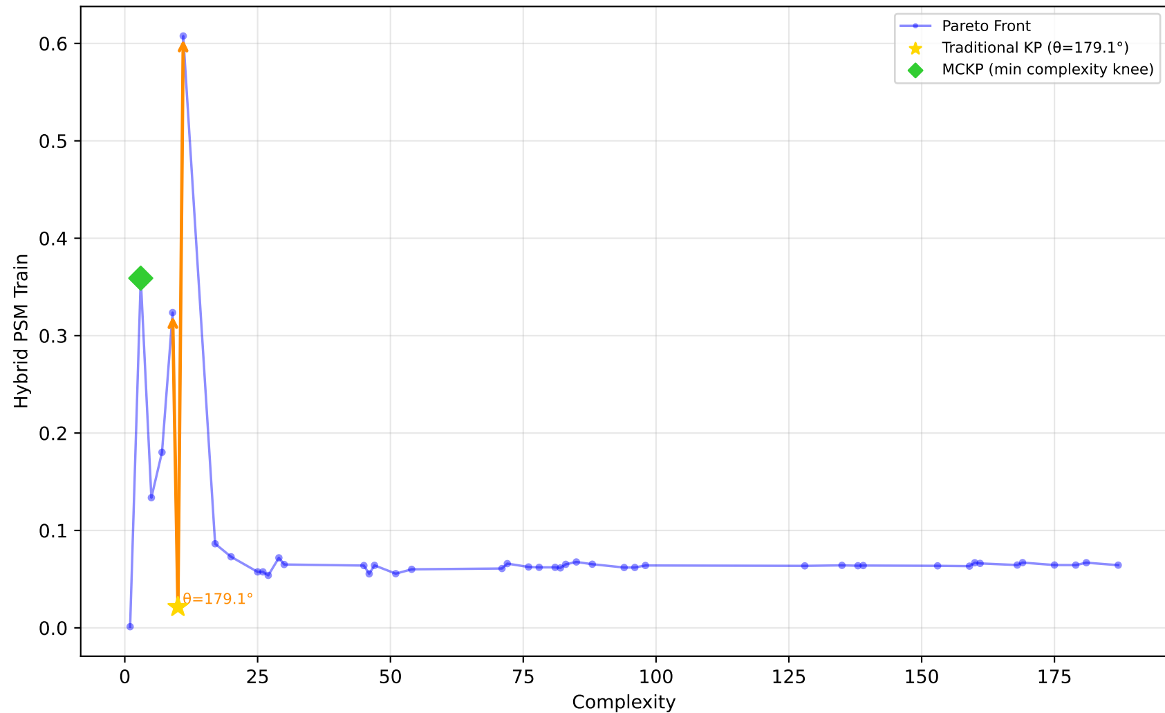
529_pollen - Run 5 - MVP - Hybrid PSM Train \lambda_1=0.00, \lambda_2=1.00, \lambda_3=0.80 | Difficulty: 1.00 | Method: hmr
