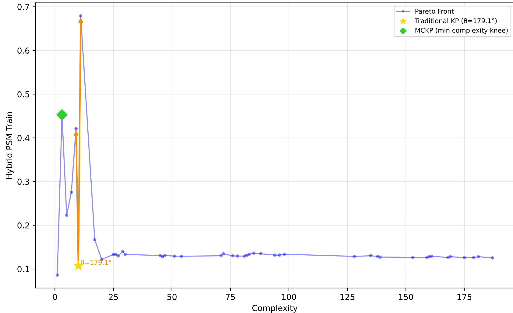
529_pollen - Run 5 - MVP - Hybrid PSM Train \lambda_1=0.90, \lambda_2=0.00, \lambda_3=0.00 | Difficulty: 1.00 | Method: hmr
