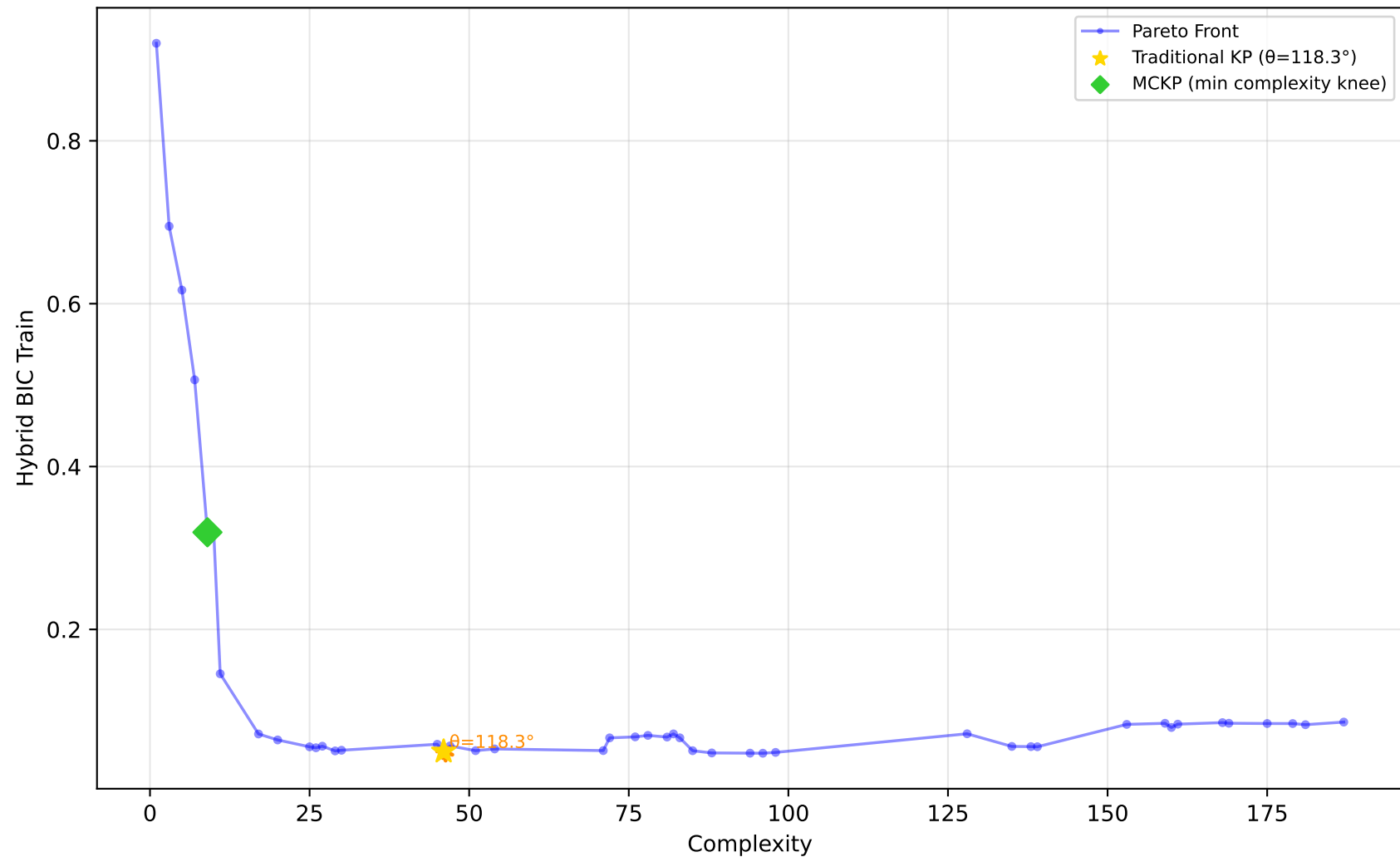
529_pollen - Run 5 - SVP - Hybrid BIC Train \lambda_1=0.10, \lambda_2=0.80, \lambda_3=0.30 | Difficulty: 1.00 | Method: hmr
