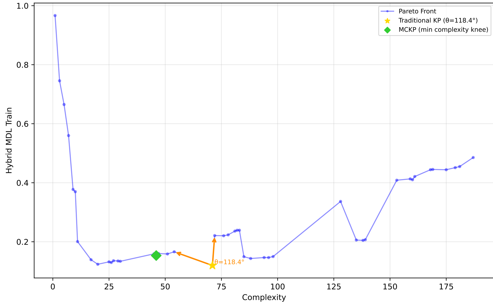
529_pollen - Run 5 - SVP - Hybrid MDL Train \lambda_1=0.60, \lambda_2=0.40, \lambda_3=1.00 | Difficulty: 1.00 | Method: hmr
