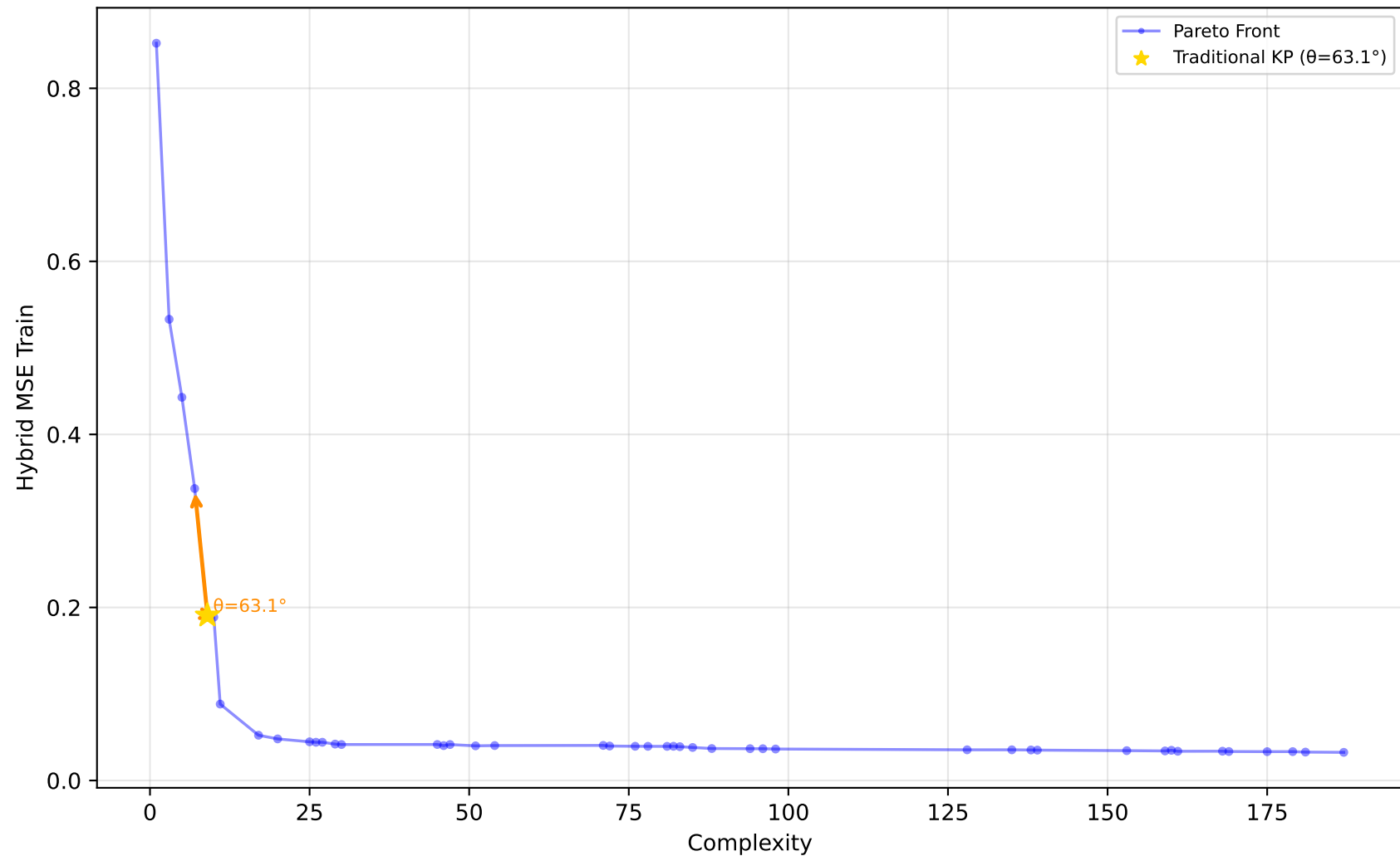
529_pollen - Run 5 - SVP - Hybrid MSE Train \lambda_1=0.10, \lambda_2=0.80, \lambda_3=0.30 | Difficulty: 1.00 | Method: hmr
