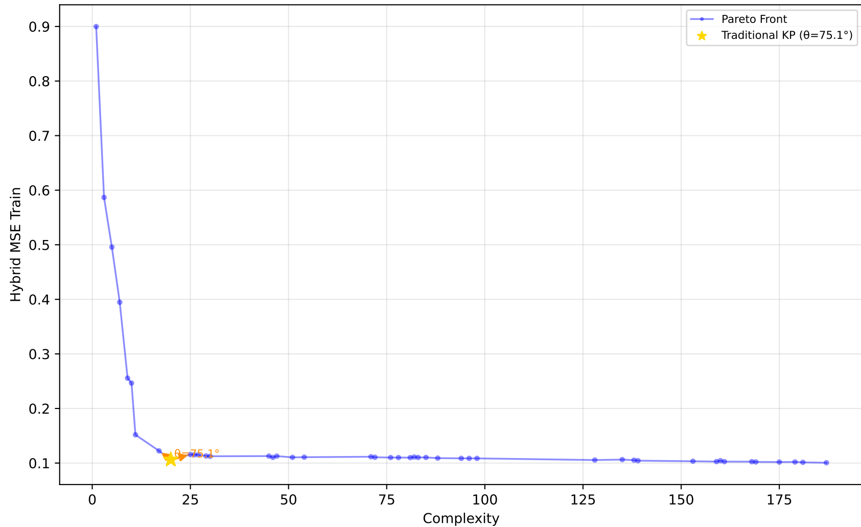
529_pollen - Run 5 - SVP - Hybrid MSE Train \lambda_1=0.60, \lambda_2=0.40, \lambda_3=1.00 | Difficulty: 1.00 | Method: hmr
