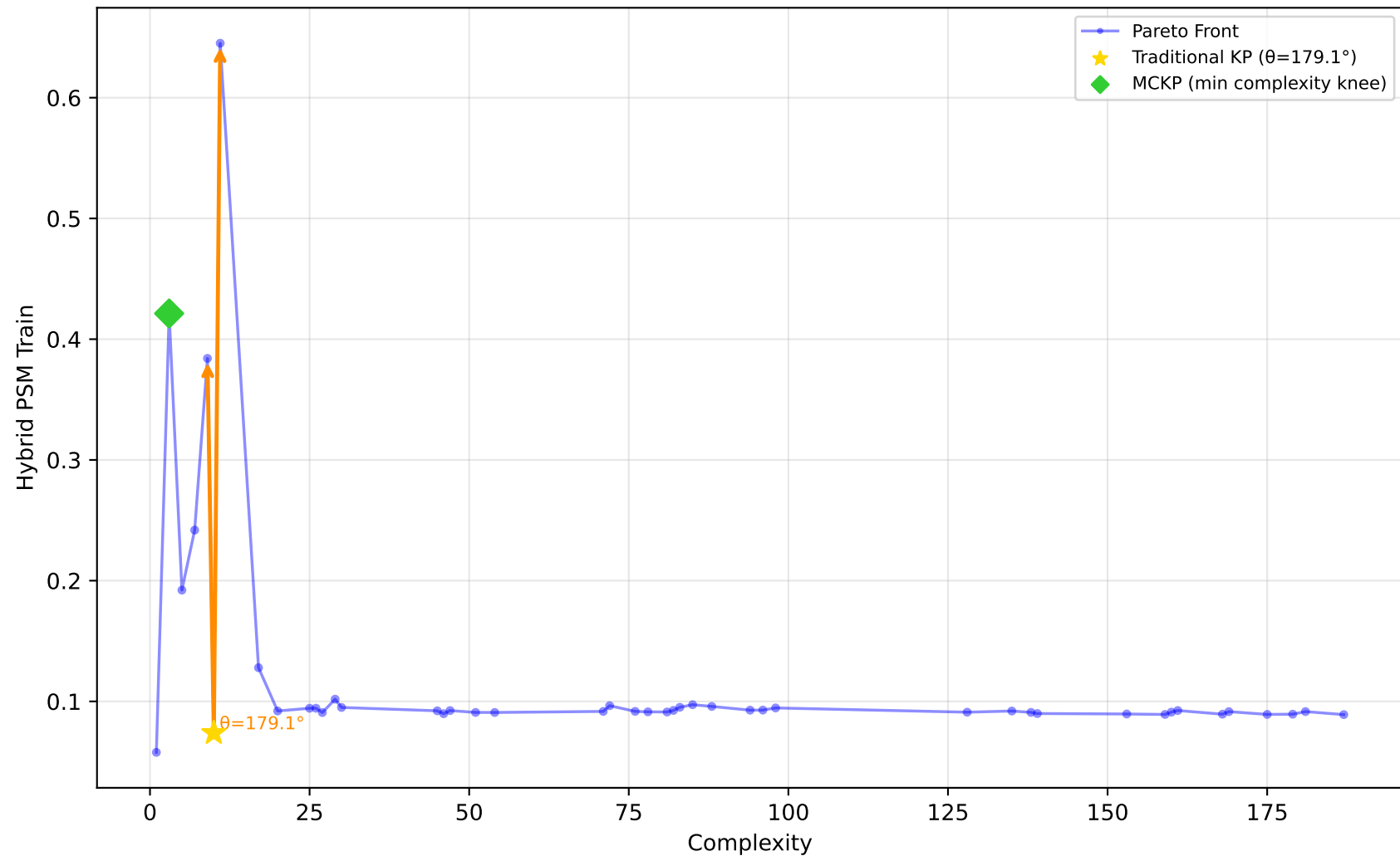
529_pollen - Run 5 - SVP - Hybrid PSM Train \lambda_1=0.60, \lambda_2=0.40, \lambda_3=1.00 | Difficulty: 1.00 | Method: hmr
