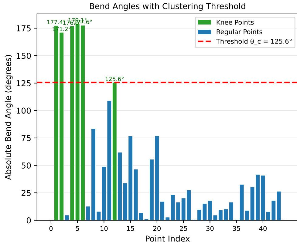
529_pollen - Run 5 - SVP - Hybrid PSM Train - Clustering Threshold \lambda_1=0.60, \lambda_2=0.40, \lambda_3=1.00 | Difficulty: 1.00
