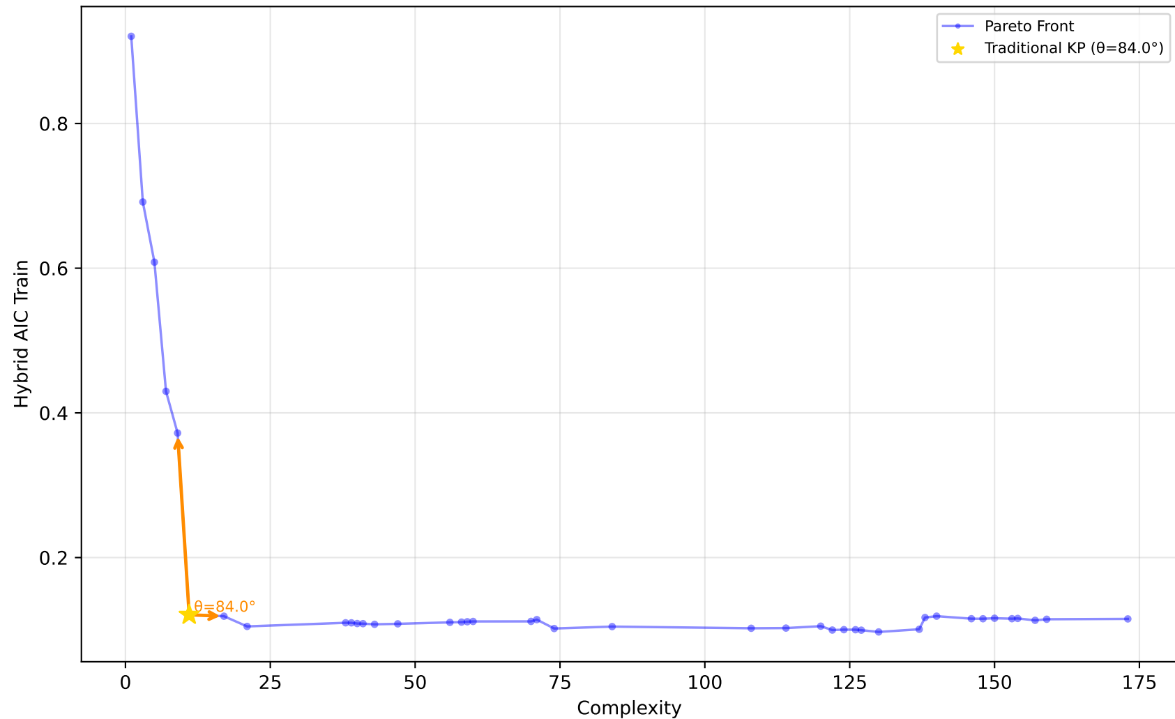
529_pollen - Run 6 - MVP - Hybrid AIC Train \lambda_1=0.00, \lambda_2=1.00, \lambda_3=0.80 | Difficulty: 1.00 | Method: hmr
