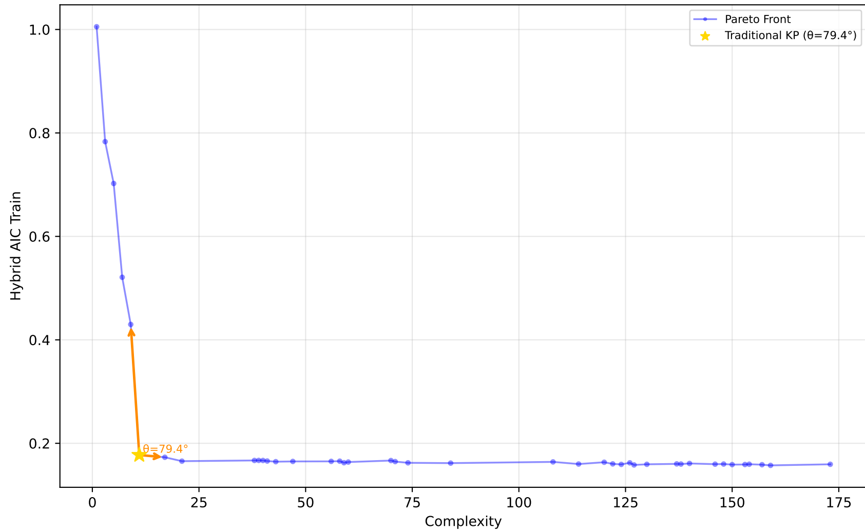
529_pollen - Run 6 - MVP - Hybrid AIC Train \lambda_1=0.90, \lambda_2=0.00, \lambda_3=0.00 | Difficulty: 1.00 | Method: hmr
