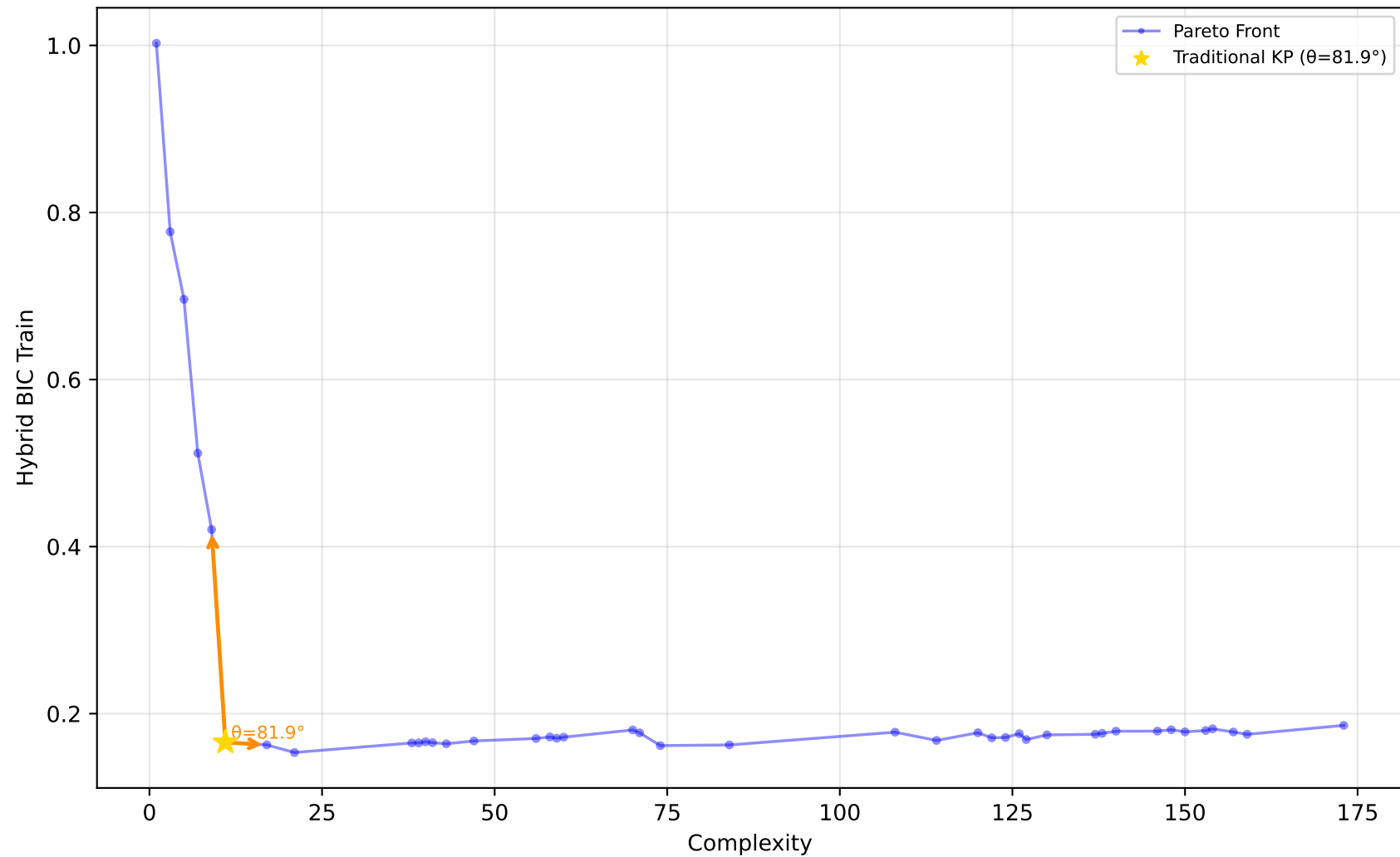
529_pollen - Run 6 - MVP - Hybrid BIC Train \lambda_1=0.90, \lambda_2=0.00, \lambda_3=0.00 | Difficulty: 1.00 | Method: hmr
