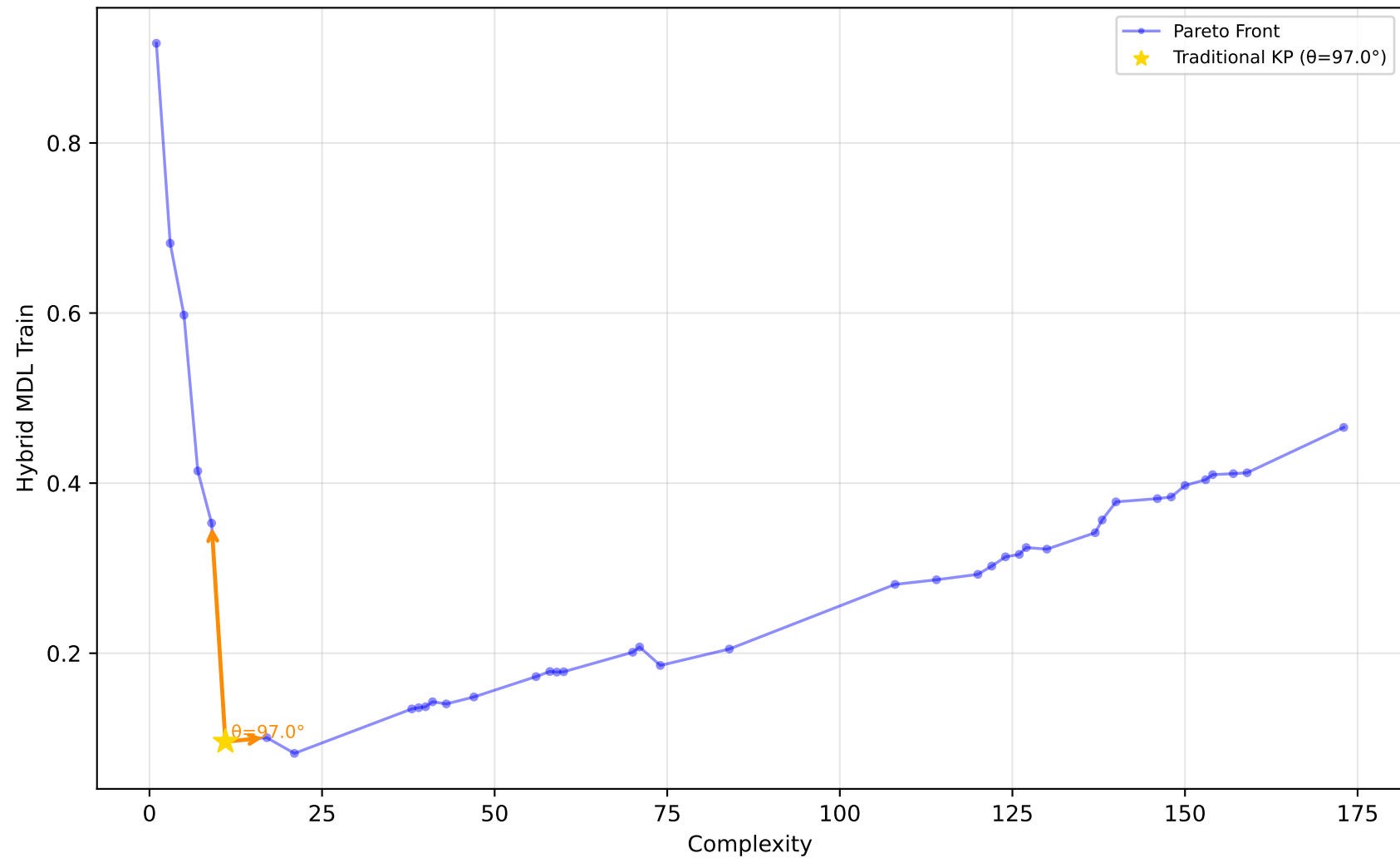
529_pollen - Run 6 - MVP - Hybrid MDL Train \lambda_1=0.00, \lambda_2=1.00, \lambda_3=0.80 | Difficulty: 1.00 | Method: hmr
