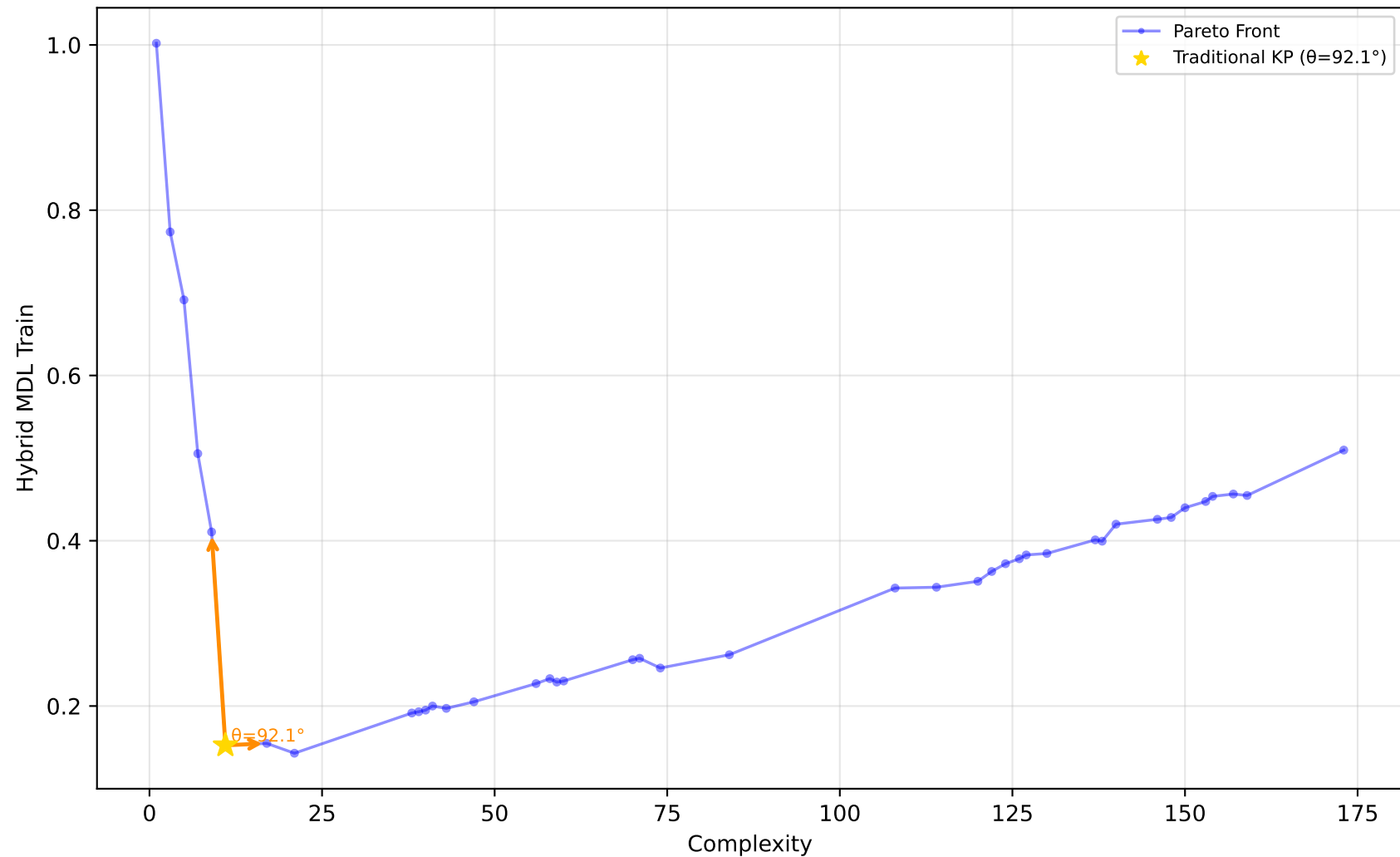
529_pollen - Run 6 - MVP - Hybrid MDL Train \lambda_1=0.90, \lambda_2=0.00, \lambda_3=0.00 | Difficulty: 1.00 | Method: hmr
