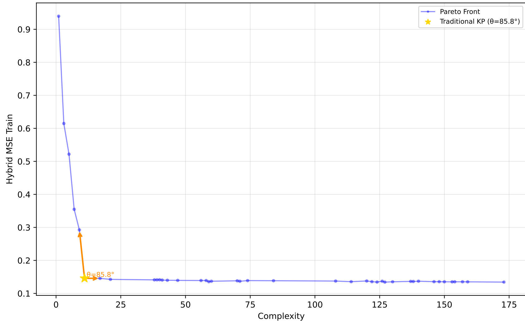
529_pollen - Run 6 - MVP - Hybrid MSE Train \lambda_1=0.90, \lambda_2=0.00, \lambda_3=0.00 | Difficulty: 1.00 | Method: hmr
