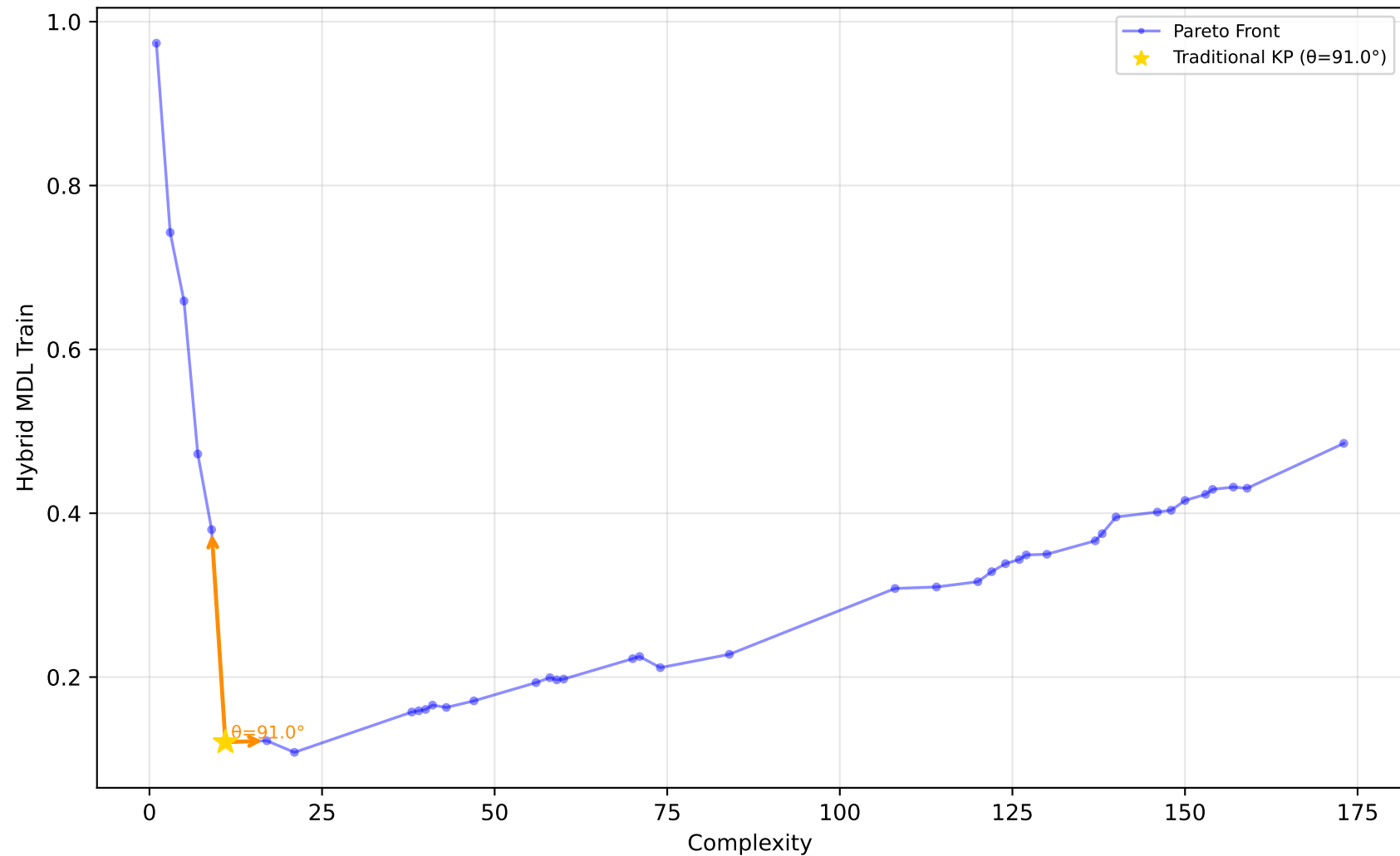
529_pollen - Run 6 - SVP - Hybrid MDL Train \lambda_1=0.60, \lambda_2=0.40, \lambda_3=1.00 | Difficulty: 1.00 | Method: hmr
