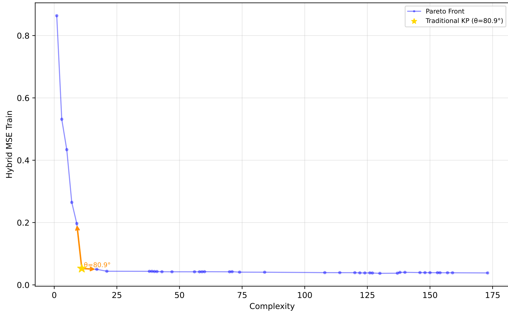
529_pollen - Run 6 - SVP - Hybrid MSE Train \lambda_1=0.10, \lambda_2=0.80, \lambda_3=0.30 | Difficulty: 1.00 | Method: hmr
