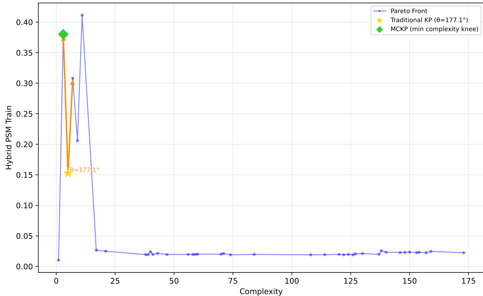
529_pollen - Run 6 - SVP - Hybrid PSM Train \lambda_1=0.10, \lambda_2=0.80, \lambda_3=0.30 | Difficulty: 1.00 | Method: hmr
