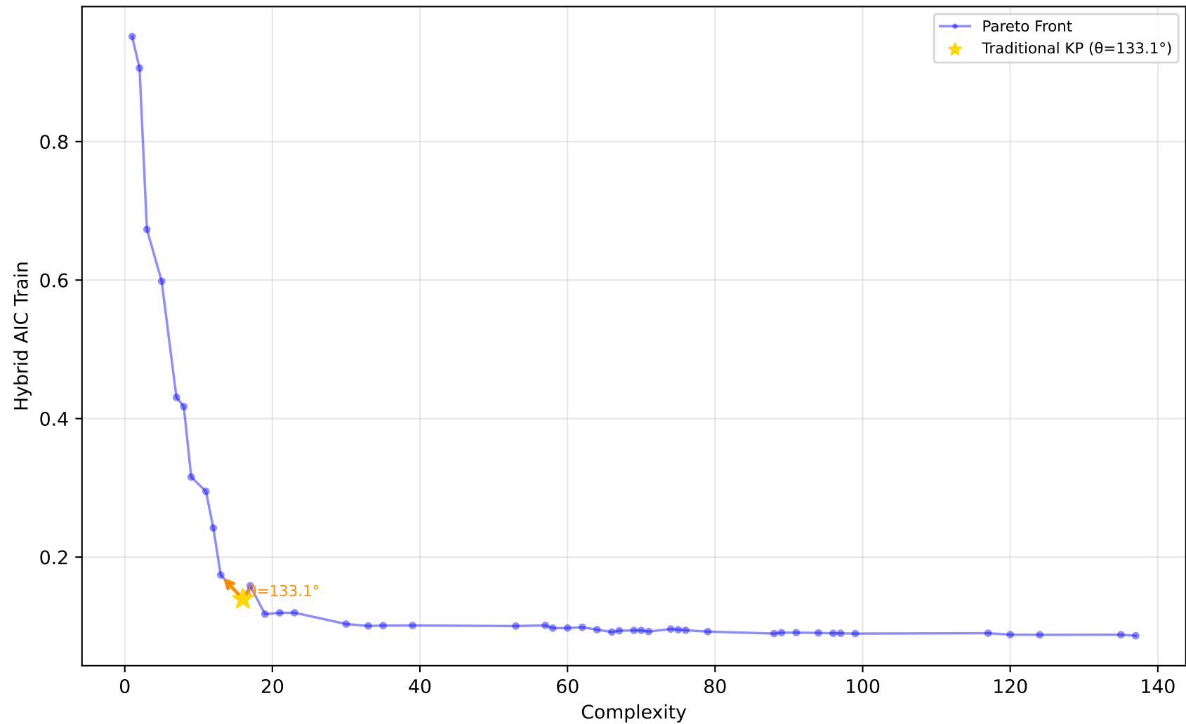
529_pollen - Run 7 - MVP - Hybrid AIC Train \lambda_1=0.00, \lambda_2=1.00, \lambda_3=0.80 | Difficulty: 1.00 | Method: hmr
