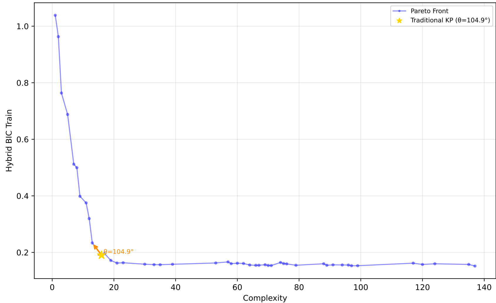
529_pollen - Run 7 - MVP - Hybrid BIC Train \lambda_1=0.90, \lambda_2=0.00, \lambda_3=0.00 | Difficulty: 1.00 | Method: hmr
