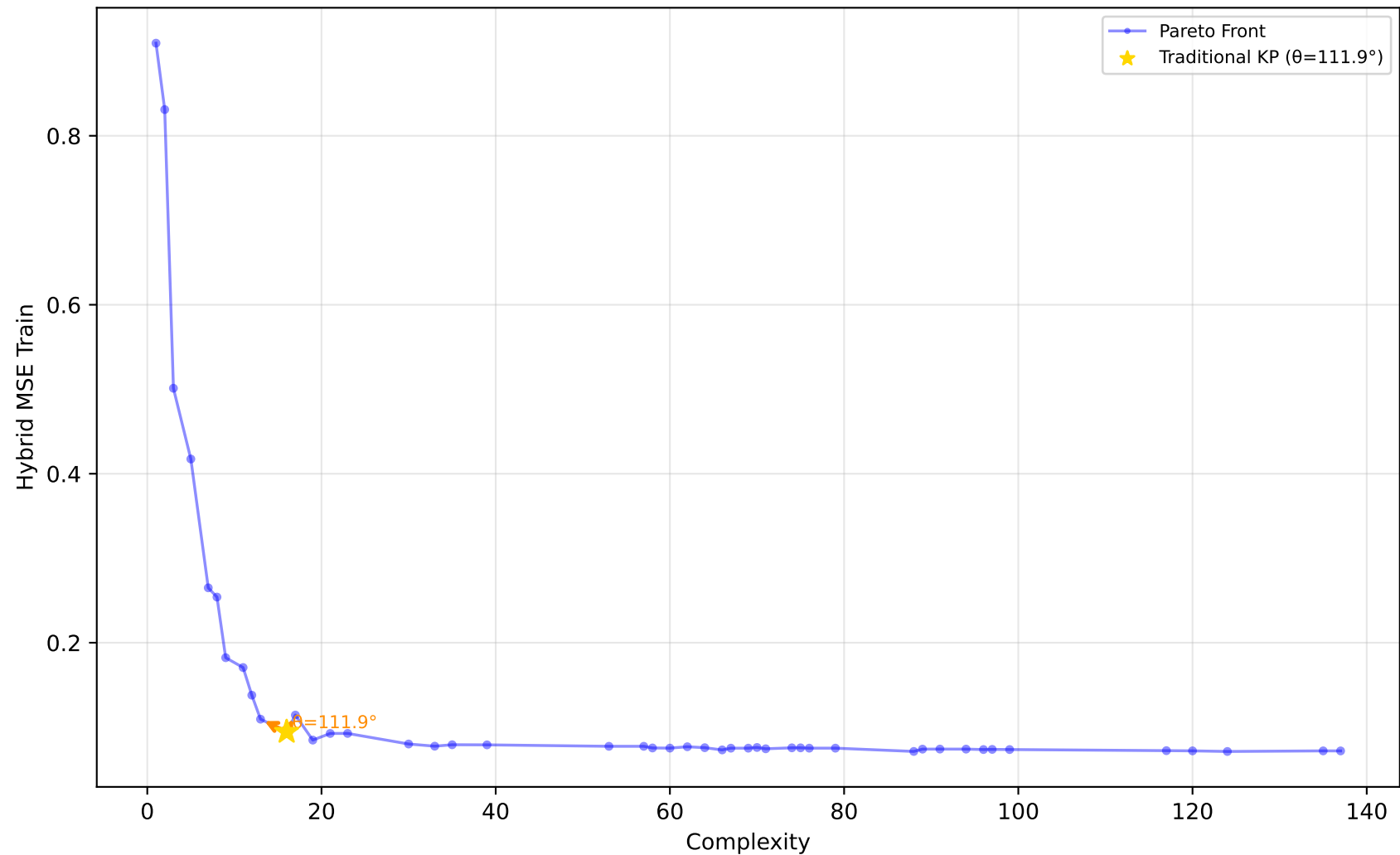
529_pollen - Run 7 - MVP - Hybrid MSE Train \lambda_1=0.00, \lambda_2=1.00, \lambda_3=0.80 | Difficulty: 1.00 | Method: hmr
