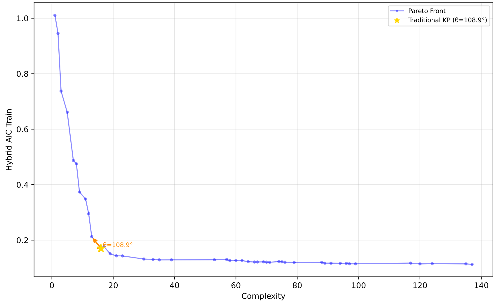
529_pollen - Run 7 - SVP - Hybrid AIC Train \lambda_1=0.60, \lambda_2=0.40, \lambda_3=1.00 | Difficulty: 1.00 | Method: hmr
