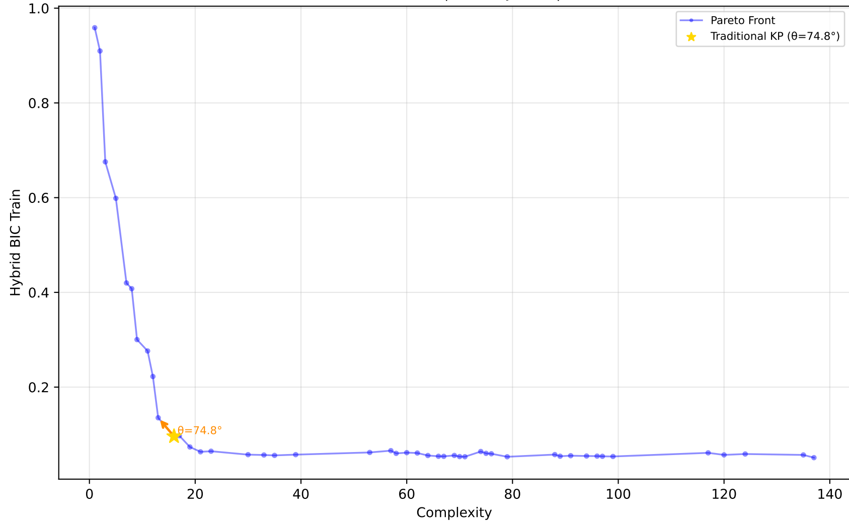
529_pollen - Run 7 - SVP - Hybrid BIC Train \lambda_1=0.10, \lambda_2=0.80, \lambda_3=0.30 | Difficulty: 1.00 | Method: hmr
