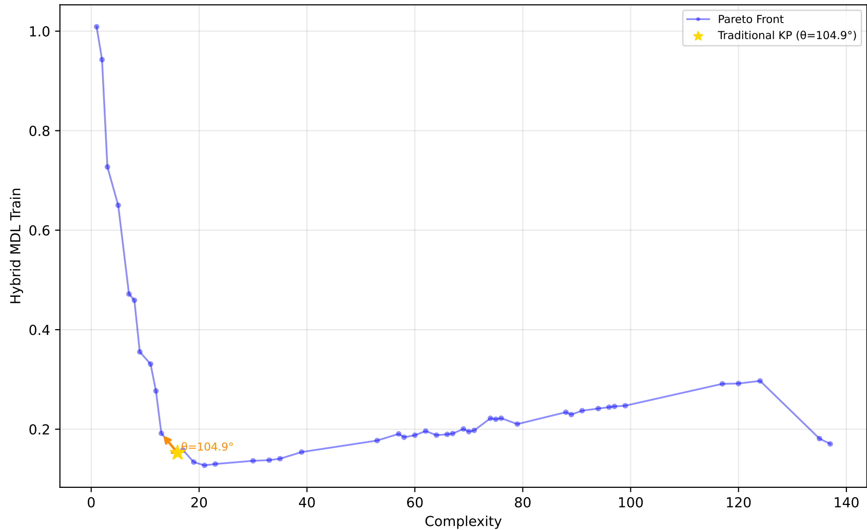
529_pollen - Run 7 - SVP - Hybrid MDL Train \lambda_1=0.60, \lambda_2=0.40, \lambda_3=1.00 | Difficulty: 1.00 | Method: hmr
