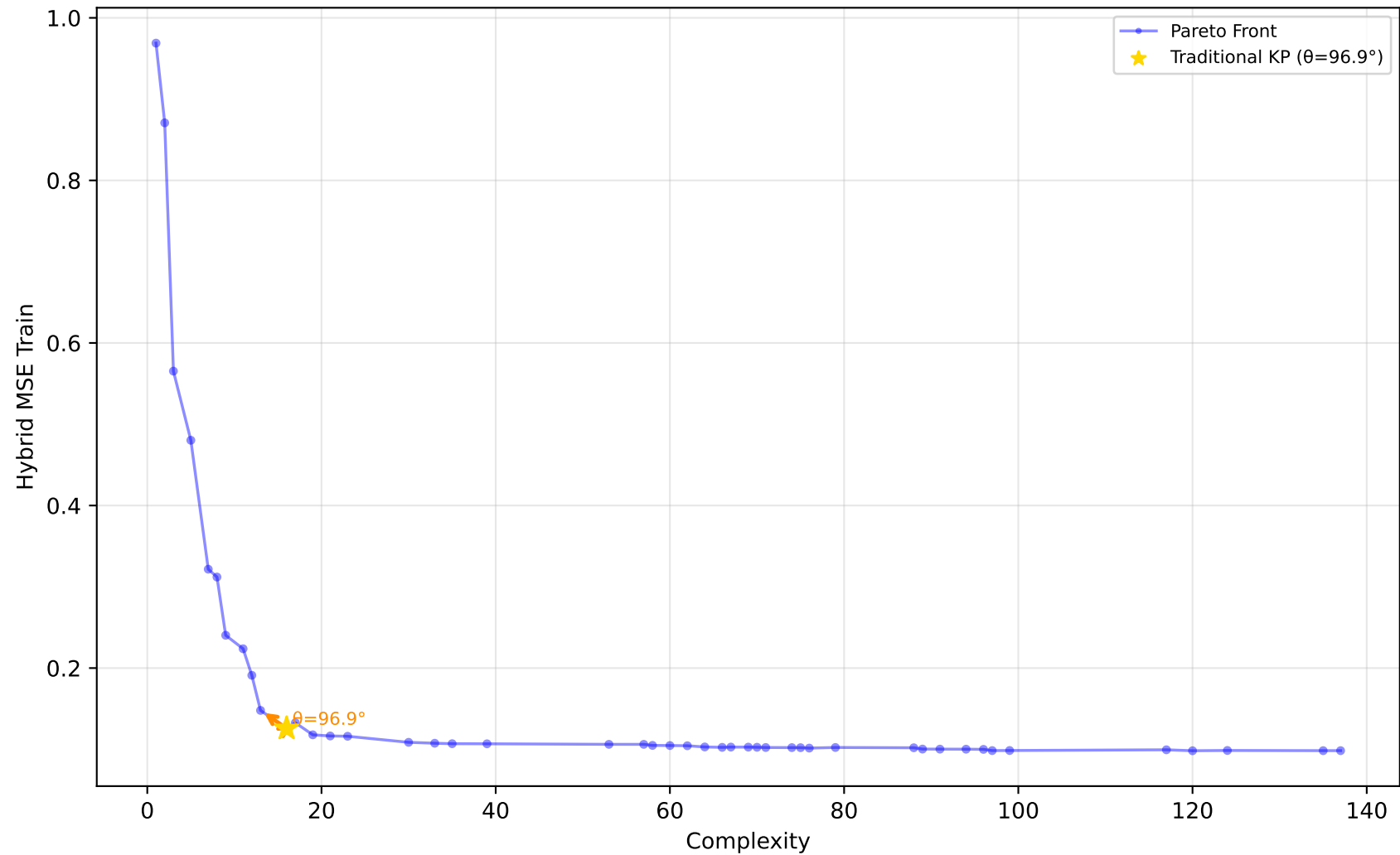
529_pollen - Run 7 - SVP - Hybrid MSE Train \lambda_1=0.60, \lambda_2=0.40, \lambda_3=1.00 | Difficulty: 1.00 | Method: hmr
