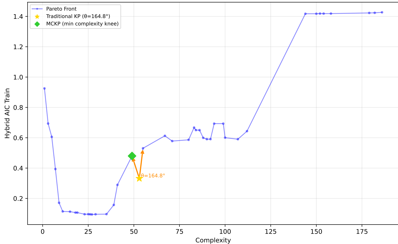
529_pollen - Run 8 - MVP - Hybrid AIC Train \lambda_1=0.00, \lambda_2=1.00, \lambda_3=0.80 | Difficulty: 0.81 | Method: hmr
