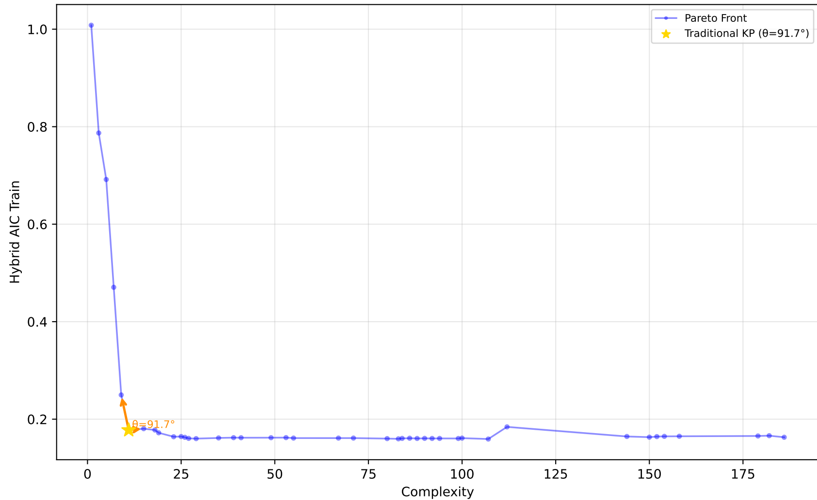
529_pollen - Run 8 - MVP - Hybrid AIC Train \lambda_1=0.90, \lambda_2=0.00, \lambda_3=0.00 | Difficulty: 0.81 | Method: hmr
