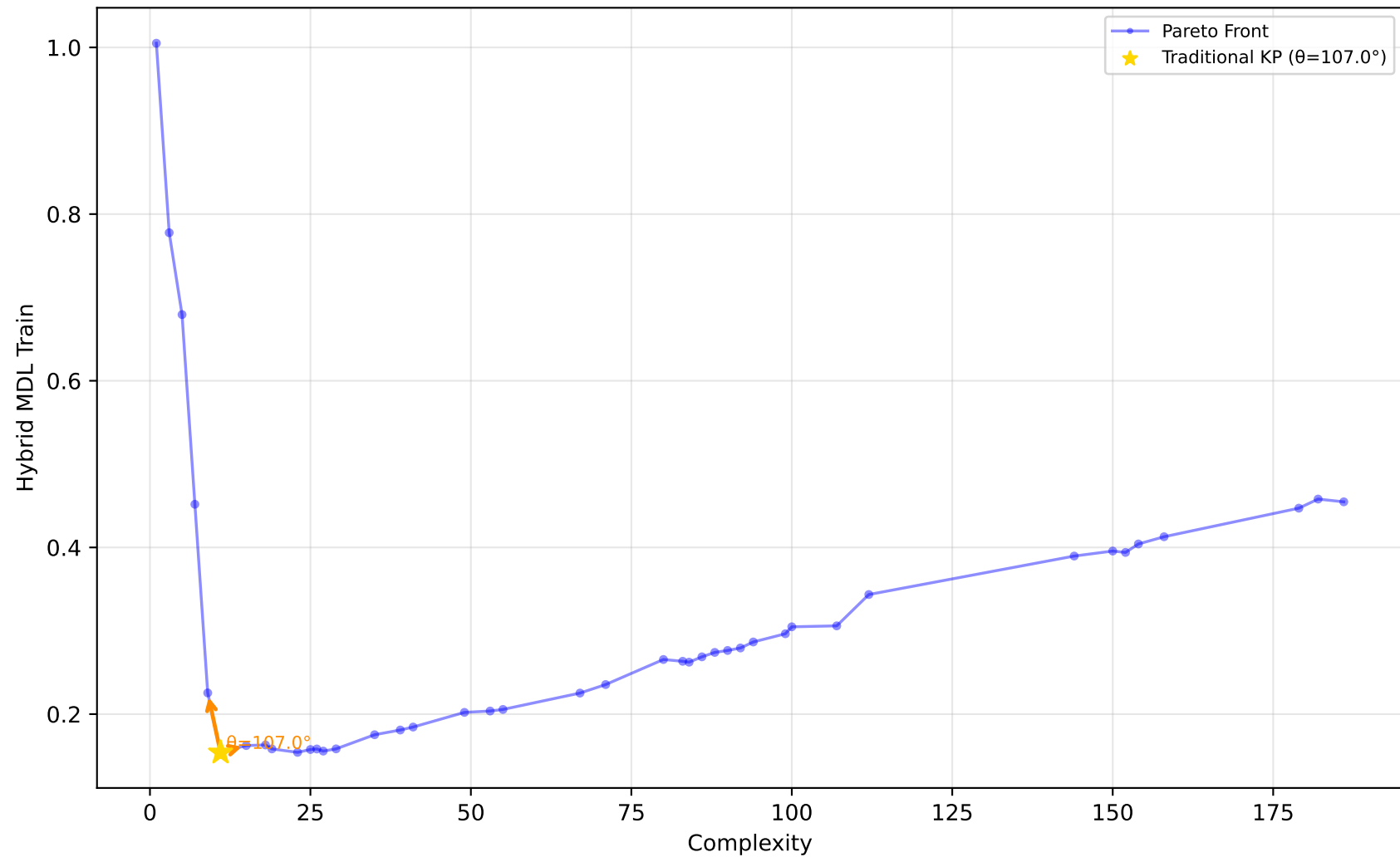
529_pollen - Run 8 - MVP - Hybrid MDL Train \lambda_1=0.90, \lambda_2=0.00, \lambda_3=0.00 | Difficulty: 0.81 | Method: hmr
